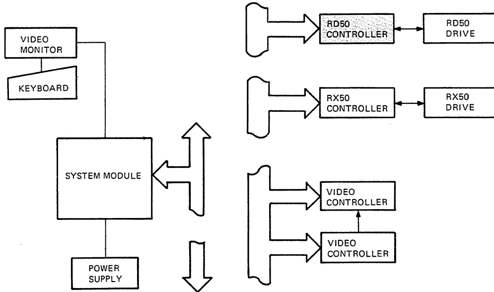
Figure 11-1 RD50 Module System Relation
