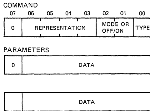
Figure 6-11 System Module to Keyboard Protocol
