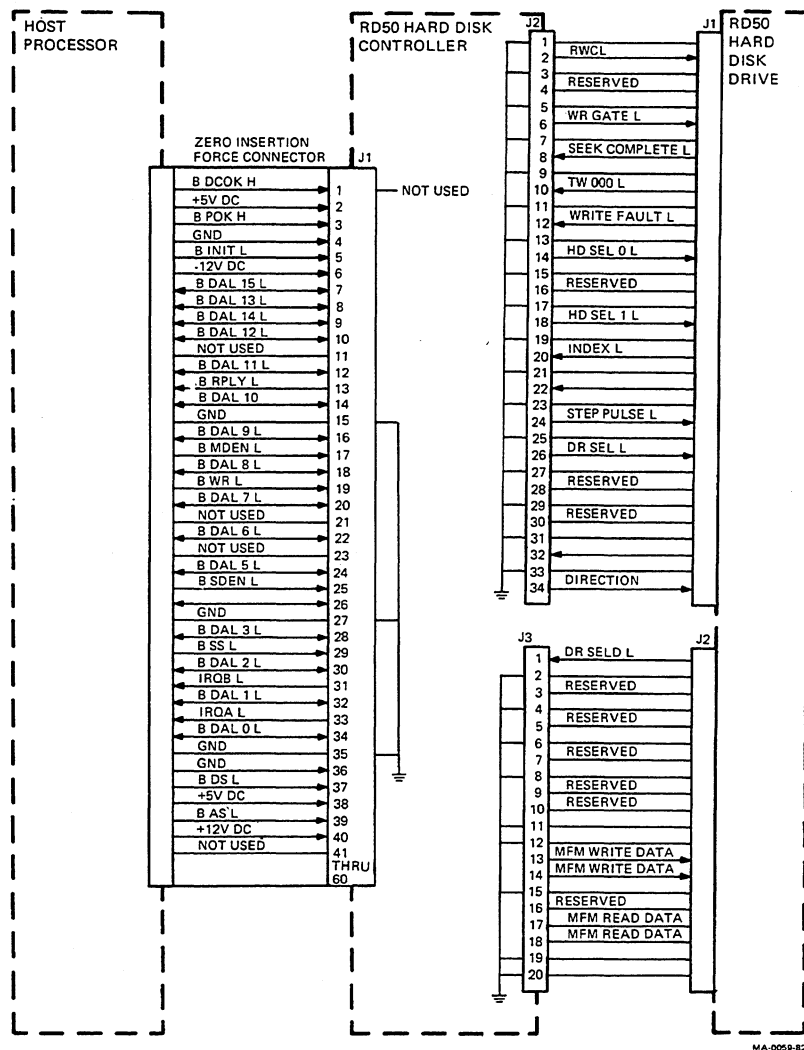
Figure 11-10 RD50 Controller Interface Signal Flow
