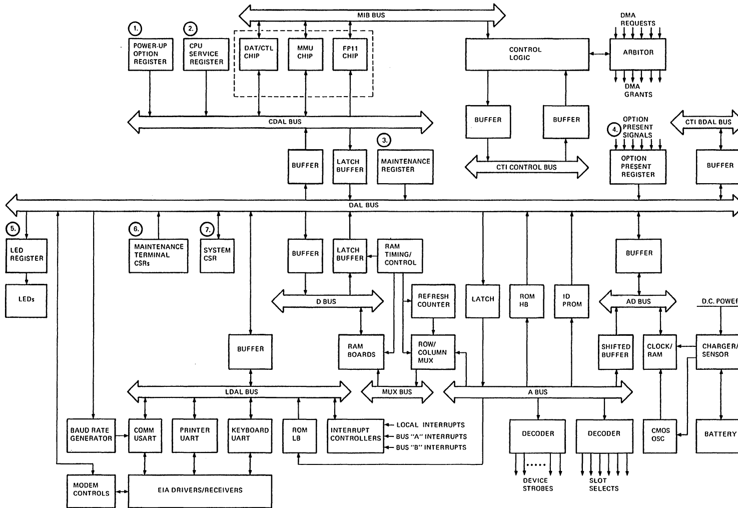
Figure 5-14 System Block Diagram with Register
