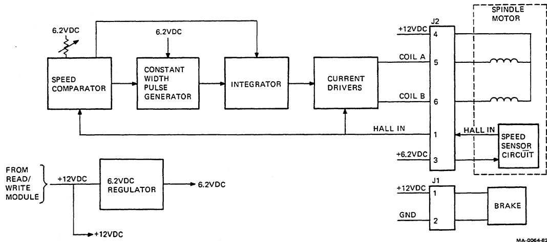
Figure 12-7 Spindle Motor Control Circuit Detail
