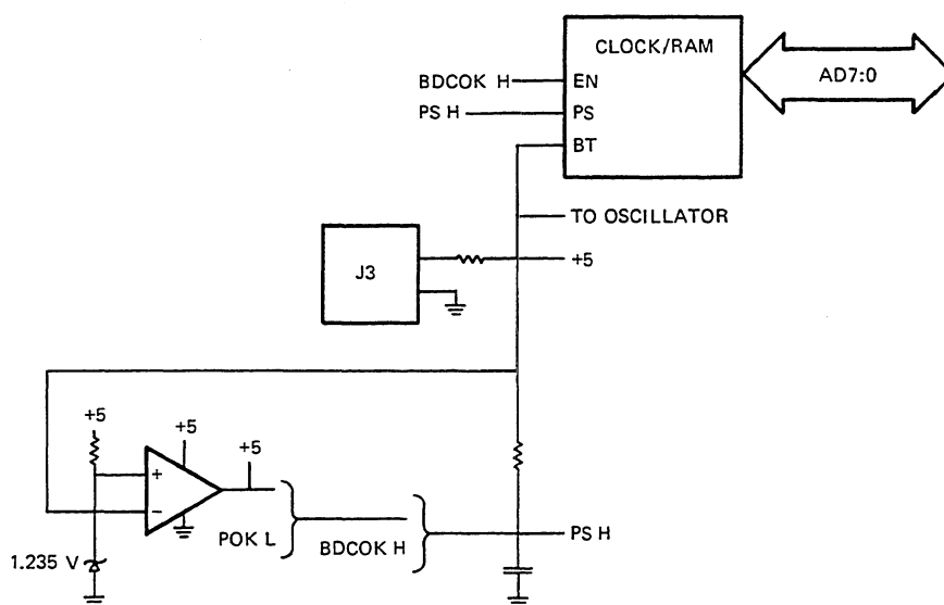
Figure 5-32 Functional Battery Charger and Voltage Sensor
