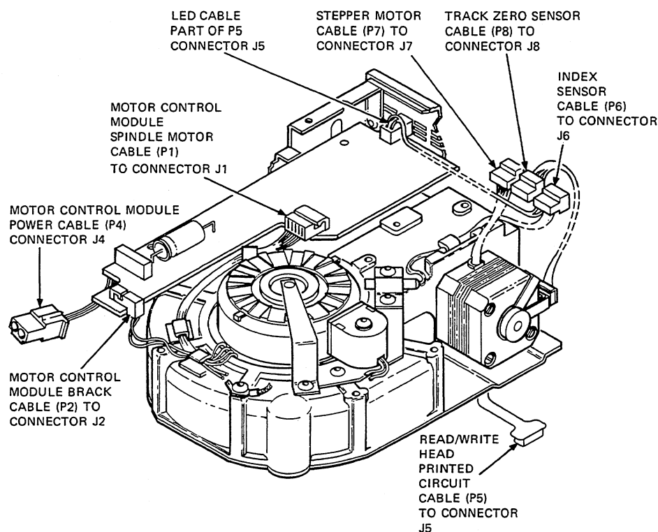
Figure 12-20 Internal Connection Locations
