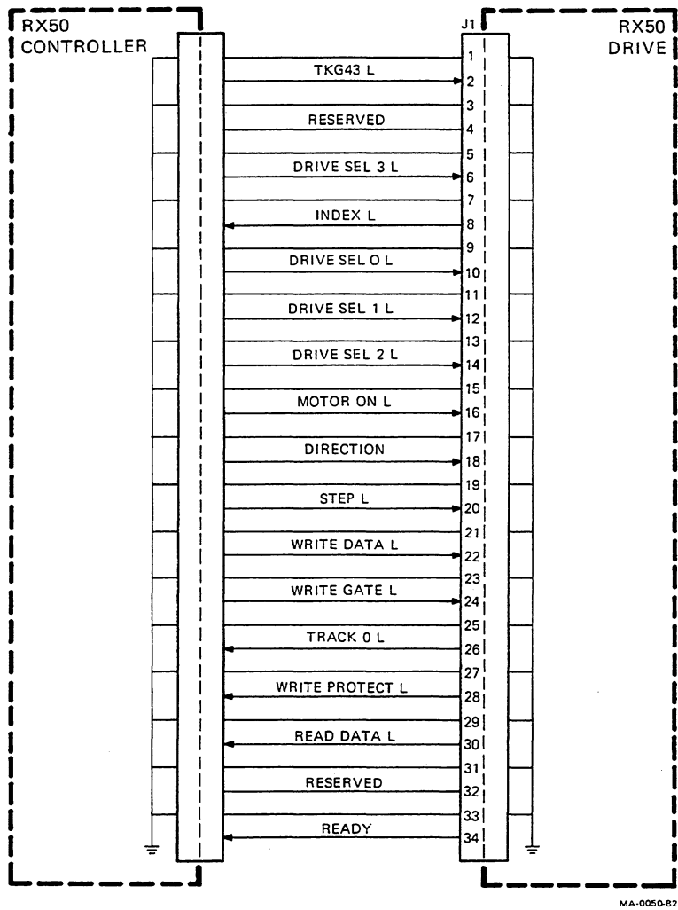
Figure 10-27 RX50 Controller and Drive Interface Signal Flow
