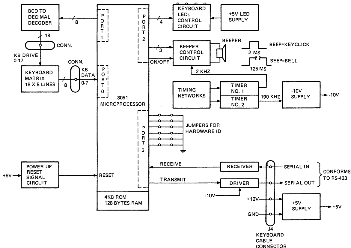
Figure 6-4 Simplified Block Diagram of LK201 Keyboard Circuitry
