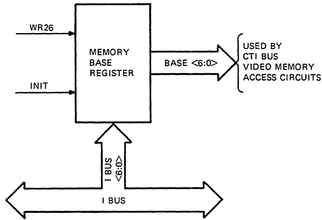
Figure 7-15 Memory Base Register Operation
