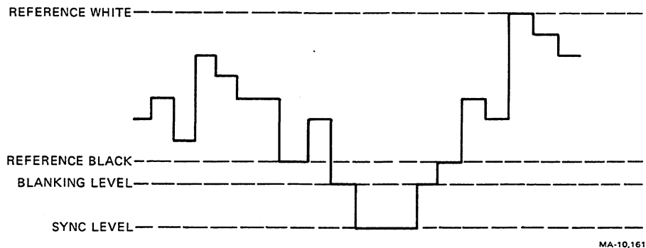
Figure 8-5 Composite Video Signal Representation
