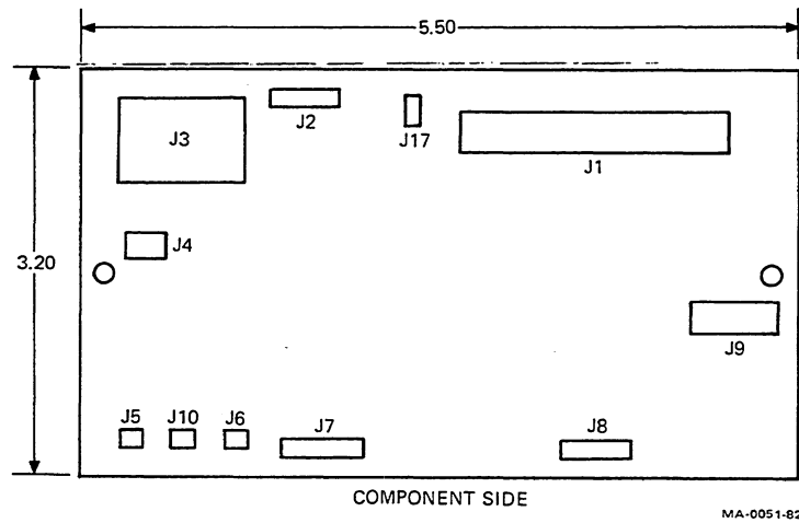
Figure 10-28 Seek and Interface Module Connector Locations
