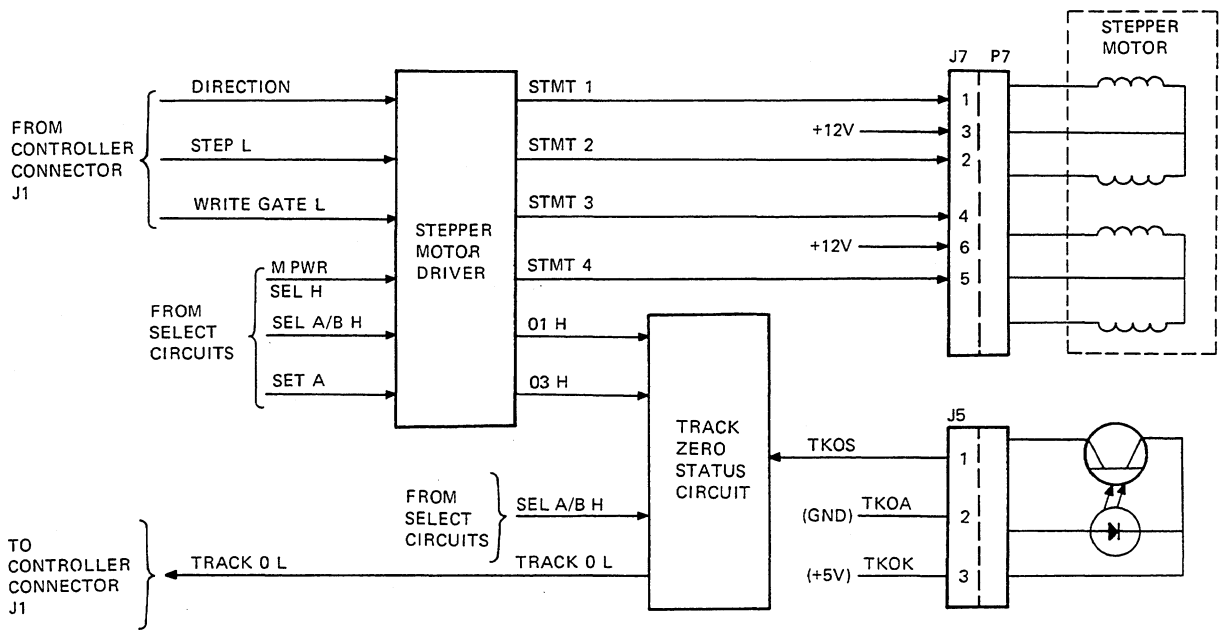
Figure 10-18 Stepper Motor Circuit Detail
