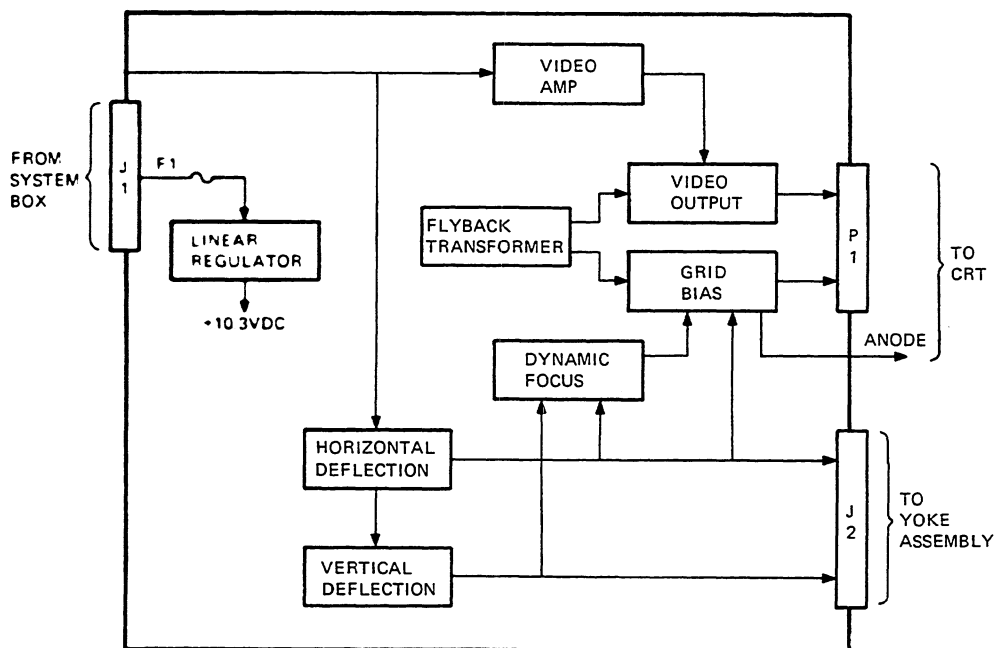
Figure 8-7 Monitor Module Block Diagram
