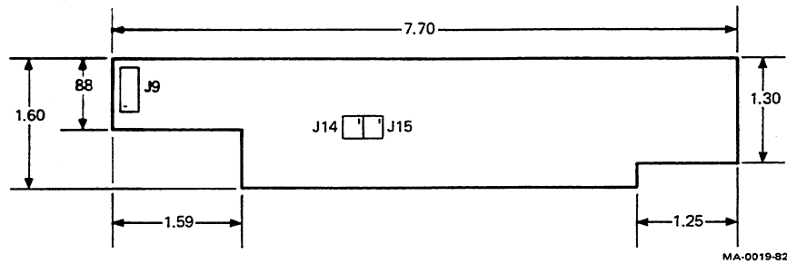
Figure 10-30 Read/Write Module Connector Locations
