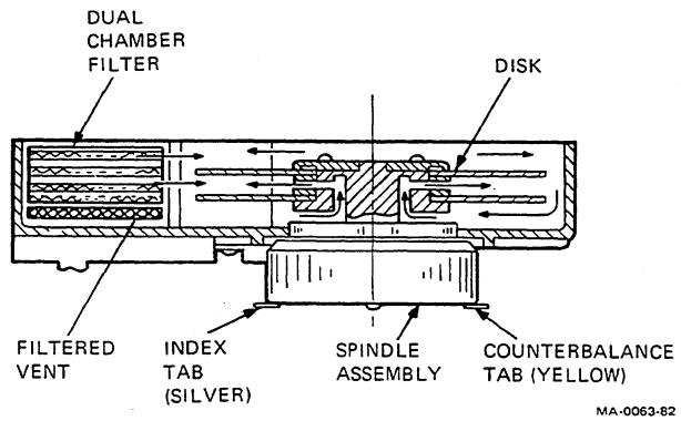
Figure 12-6 Air Flow Side View
