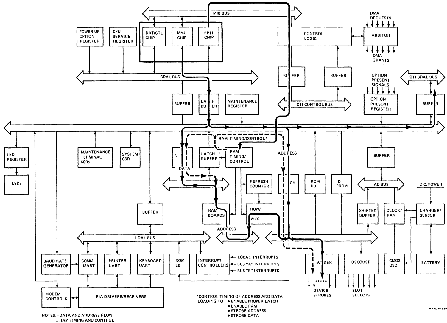
Figure 5-22 CPU Writing Out to RAM
