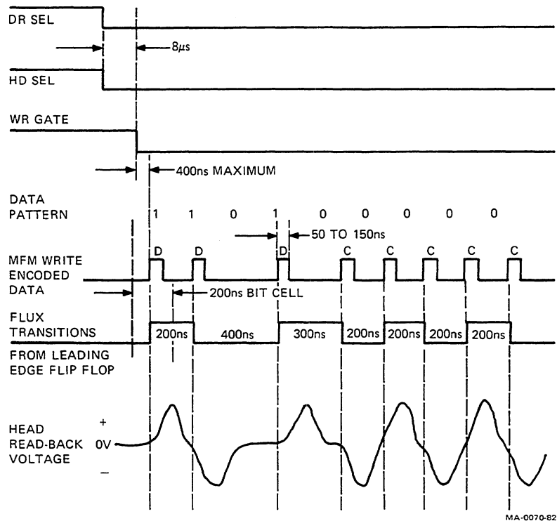
Figure 12-14 Write Data Timing
