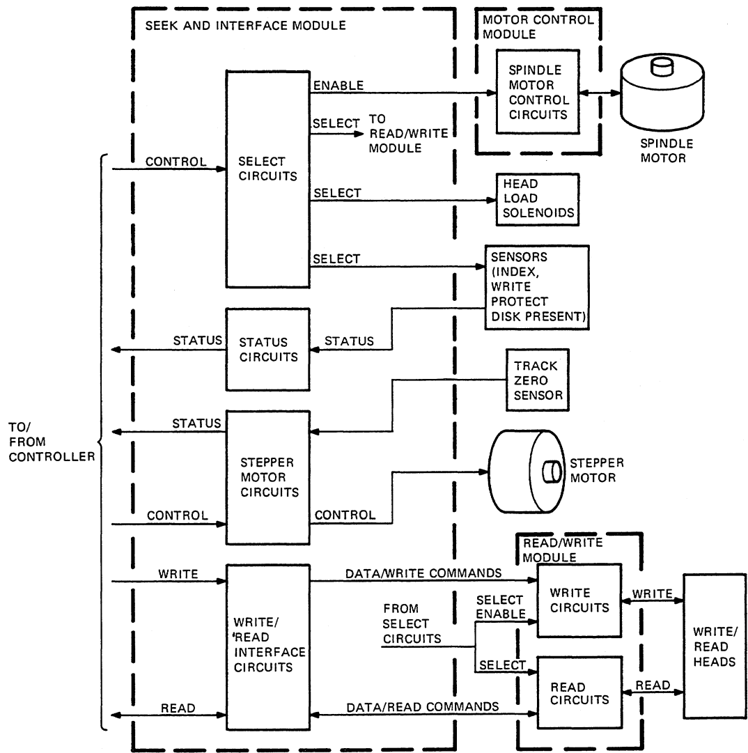
Figure 10-8 Simple Block Diagram
