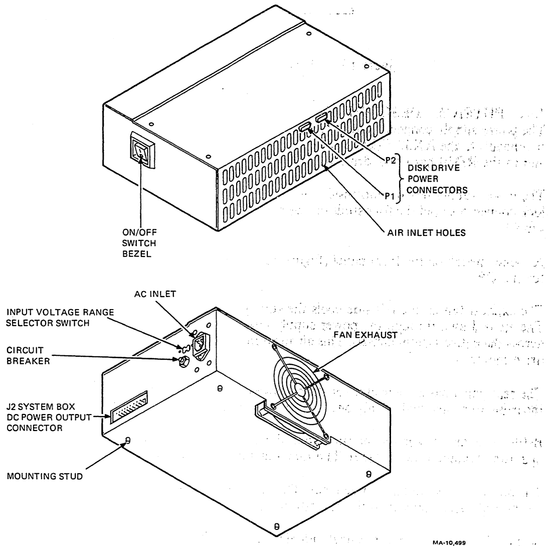
Figure 13-3 H7862 Power Supply
