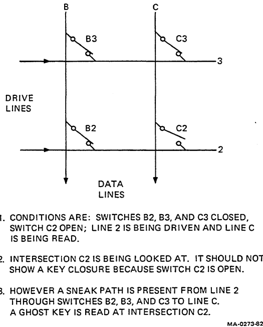
Figure 6-6 Example of Ghost Key Generation
