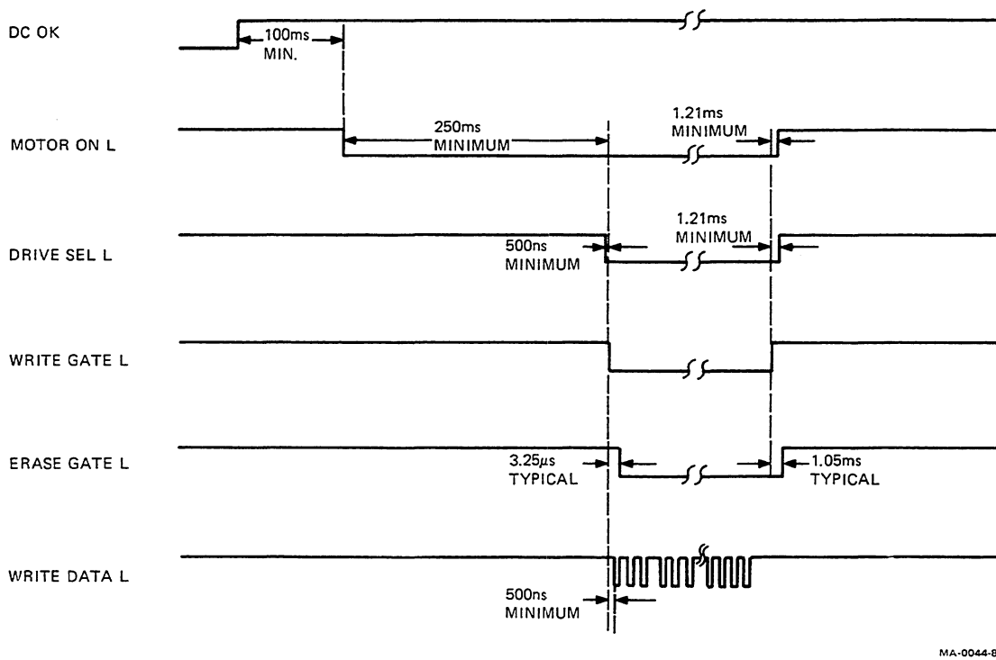
Figure 10-21 Write Data Timing Relationships
