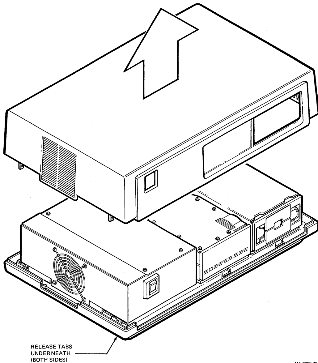
Figure 2-3 Top Cover Removal
