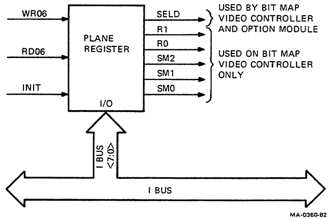
Figure 7-10 Plane Register Operation
