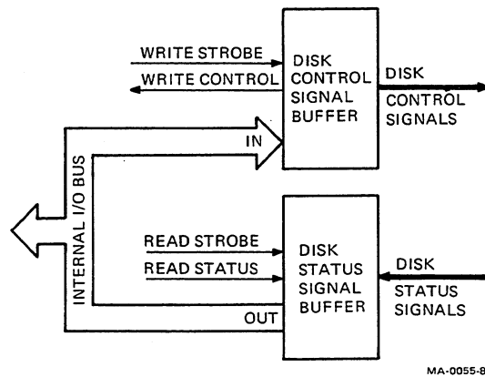
Figure 11-6 Disk Control and Status Circuits
