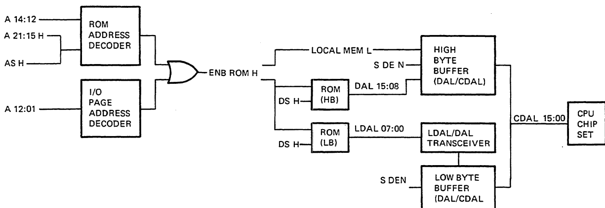
Figure 5-26 ROM Addressing and Reading
