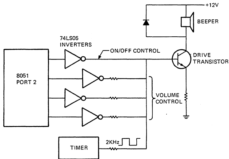
Figure 6-8 Beeper Control Circuit
