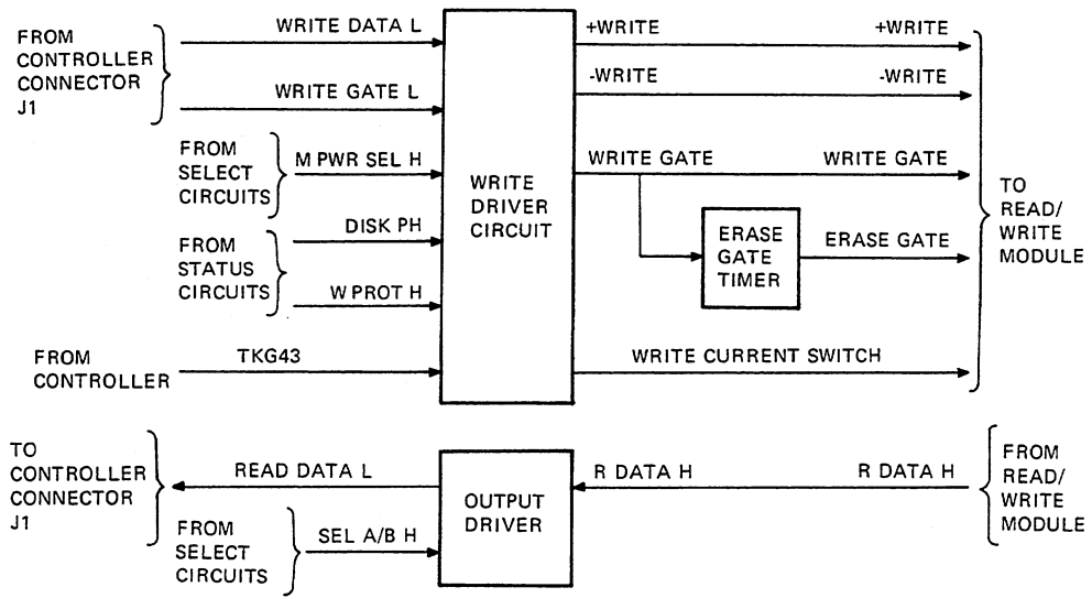
Figure 10-20 Read/Write Interface Circuit Detail
