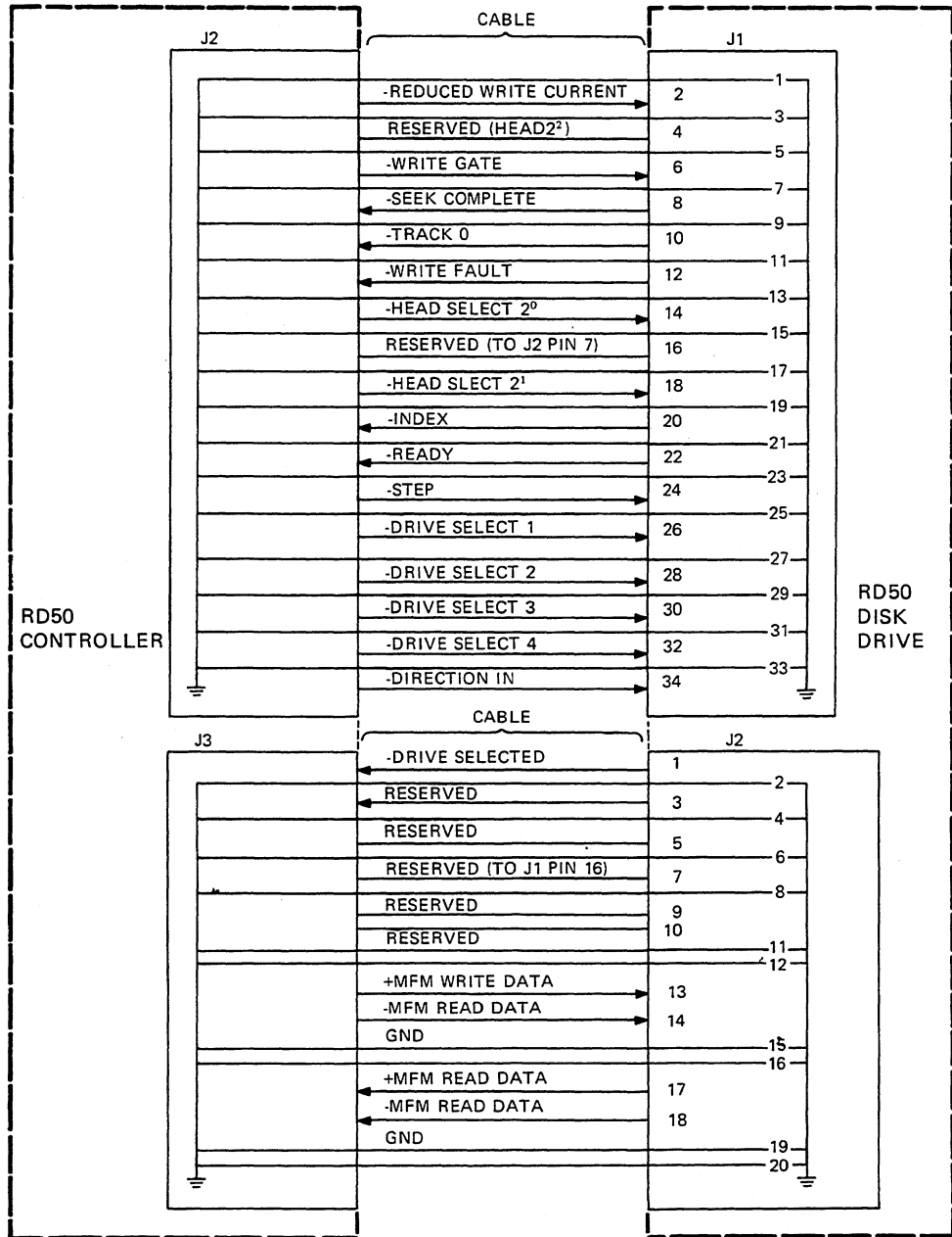
Figure 12-18 RD50 Interface Signal Connections
