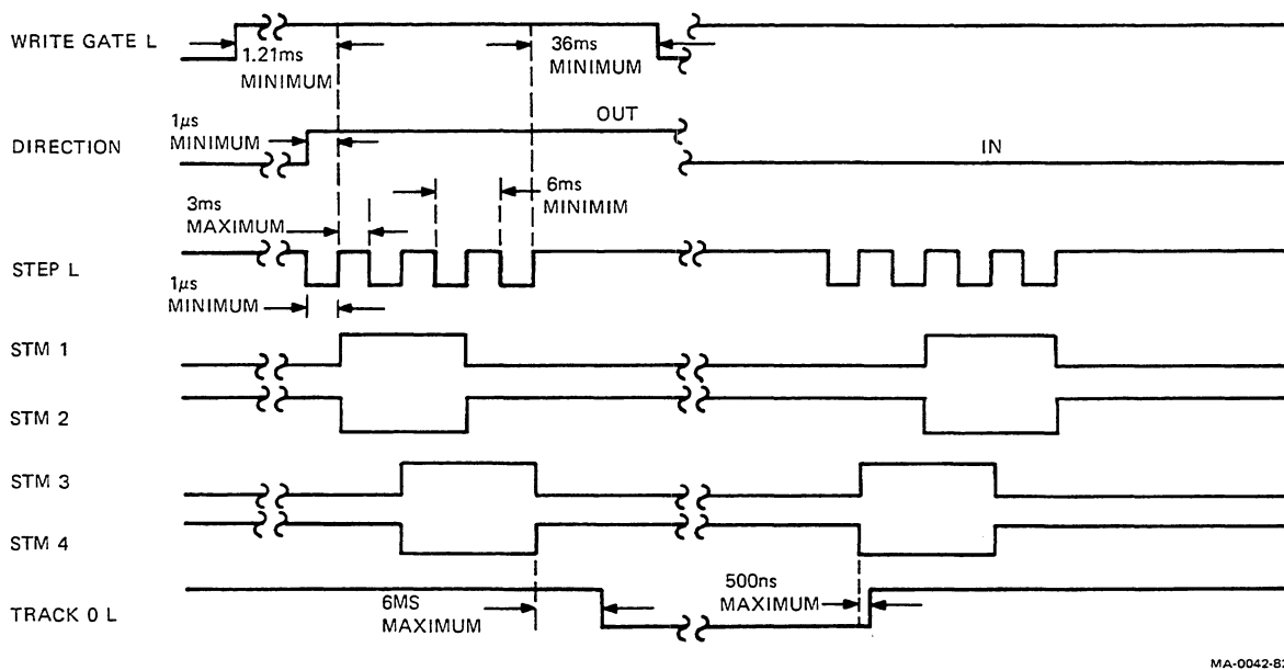
Figure 10-19 Stepper Motor Timing Relationships
