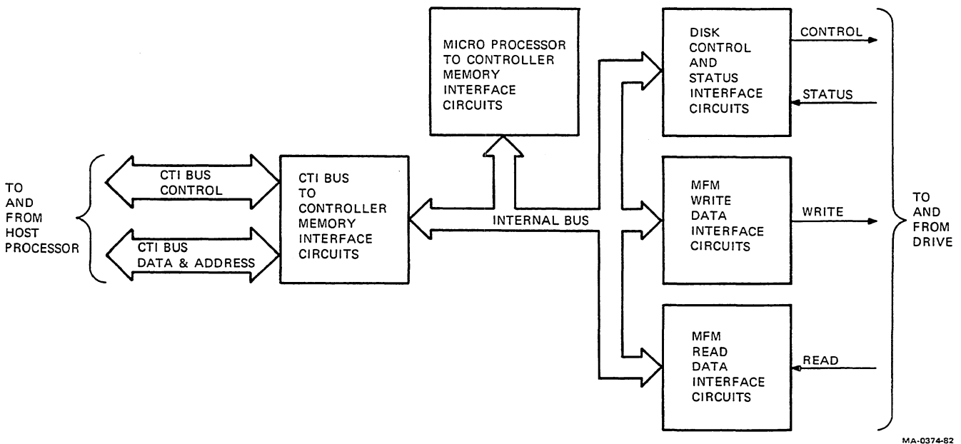
Figure 9-3 RX50 Controller Module Block Diagram
