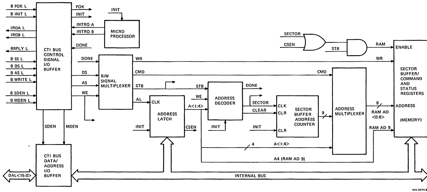
Figure 9-4 CTI BUS to Controller Memory Interface Circuits
