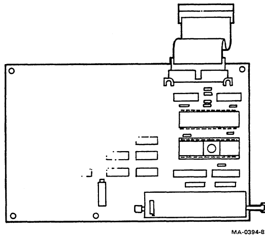
Figure 9-2 RX50 Controller Module
