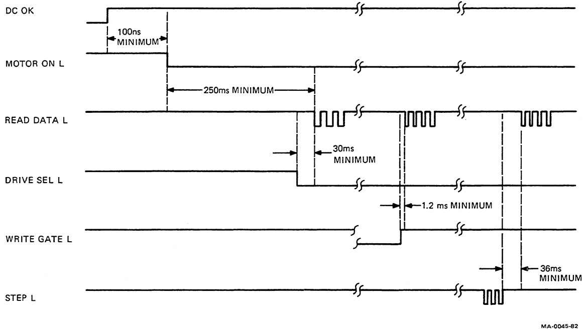
Figure 10-22 Read Data Timing Relationships
