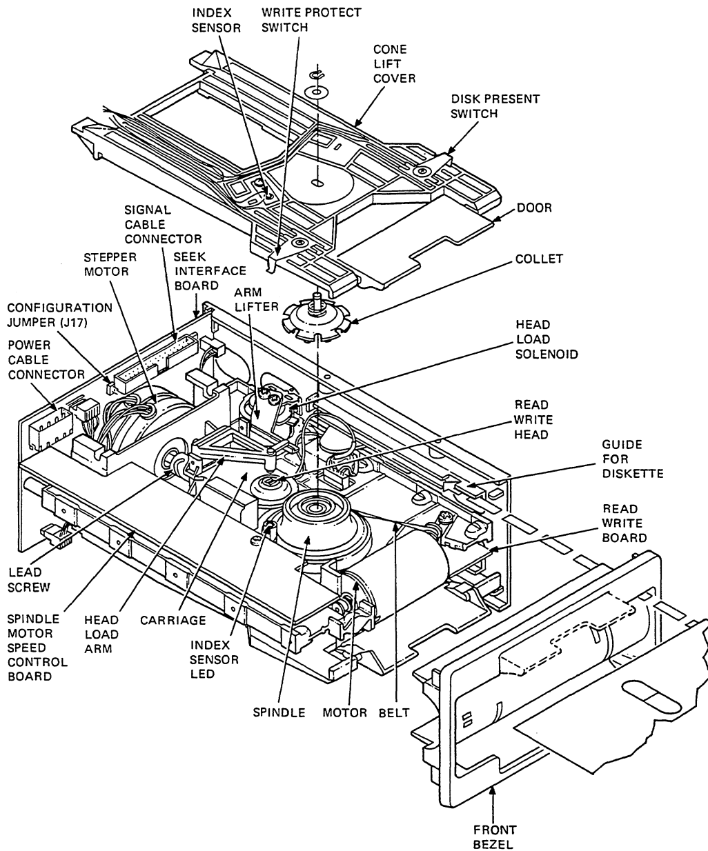
Figure 10-9 Mechanical Detail
