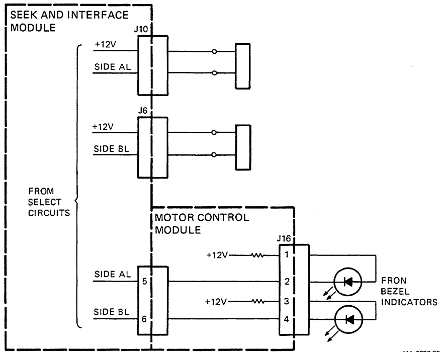
Figure 10-14 Connections to Head Load Solenoids and Indicators
