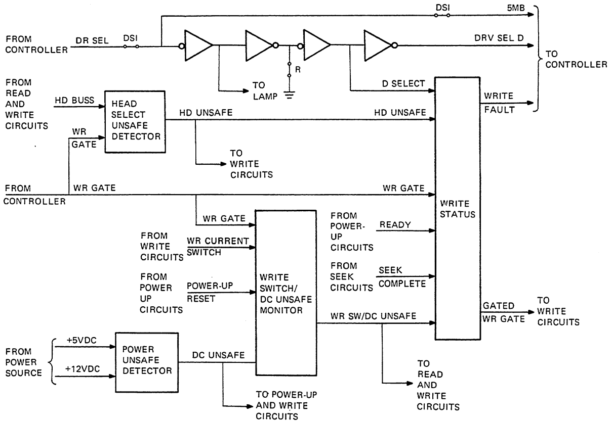
Figure 12-10 Fault Detection Circuit Detail
