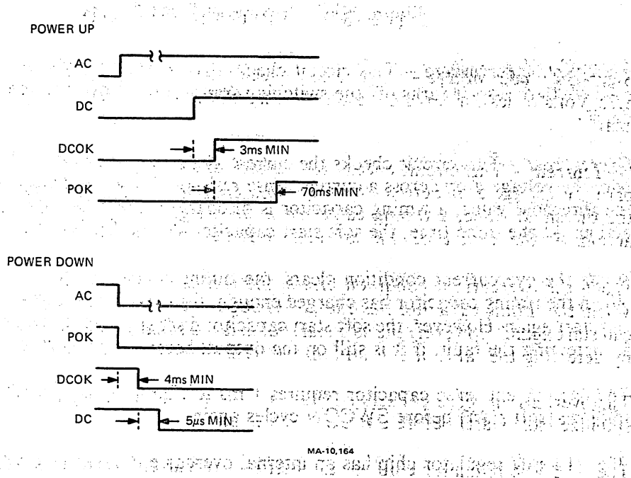
Figure 13-9 Power Status Signal Timing
