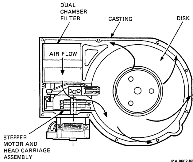
Figure 12-5 Air Flow Top View
