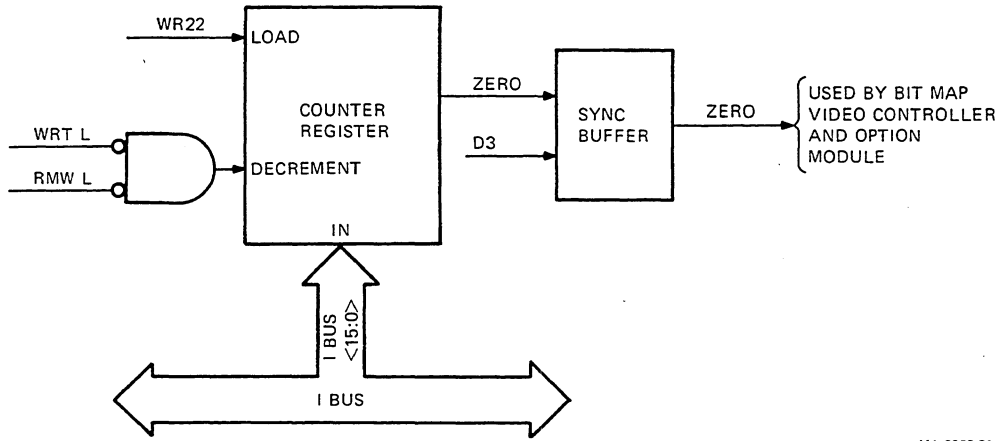
Figure 7-13 Counter Register Operation
