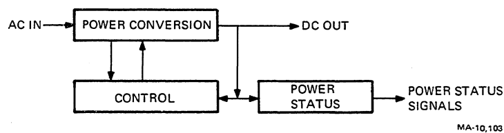
Figure 13-2 Power Supply Functional Block Diagram
