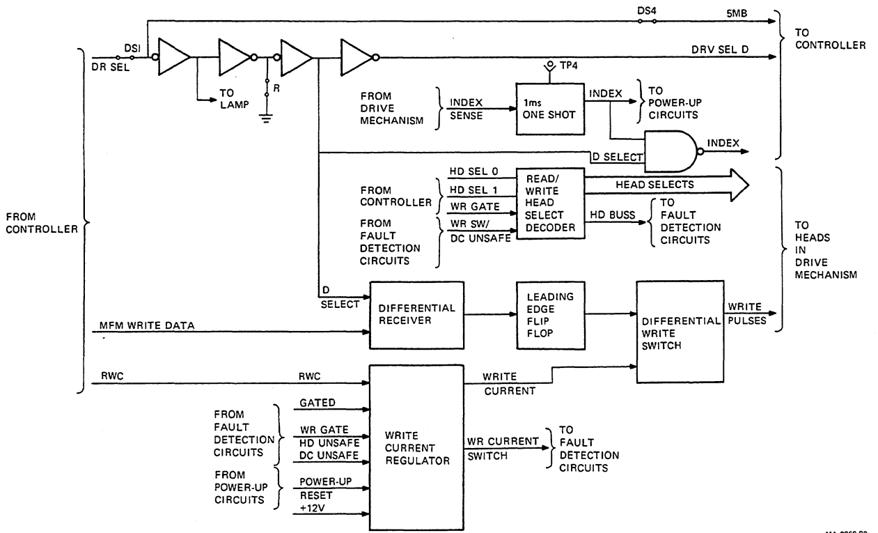
Figure 12-13 Write Circuit Detail
