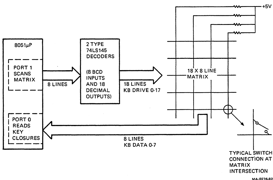
Figure 6-5 Simplified Block Diagram of Matrix Scanning Circuit
