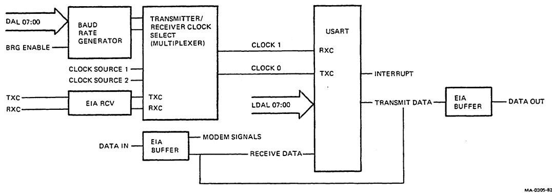
Figure 5-31 Communications Interface
