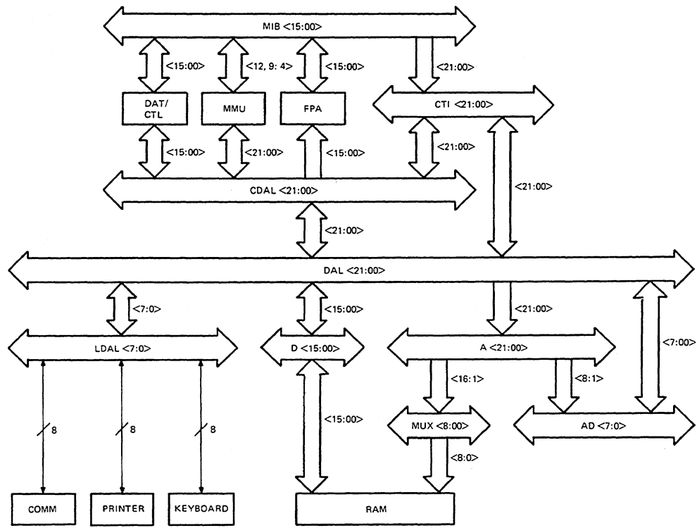
Figure 5-9 Professional 350 System Module Bus Scheme
