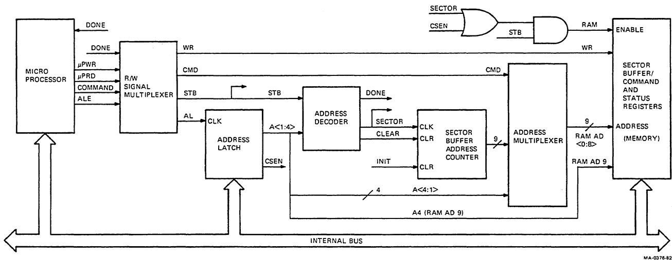
Figure 9-5 Microprocessor to Controller Memory Interface Circuits
