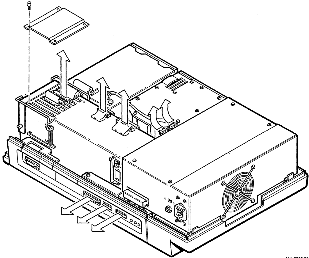
Figure 2-7 Removing the Cables
