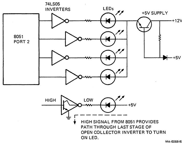
Figure 6-9 Indicator (LED) Control Circuit
