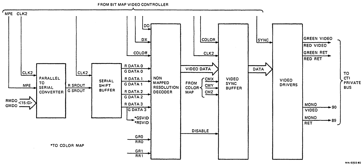
Figure 7-28 Video Generator Operation (Option Module)
