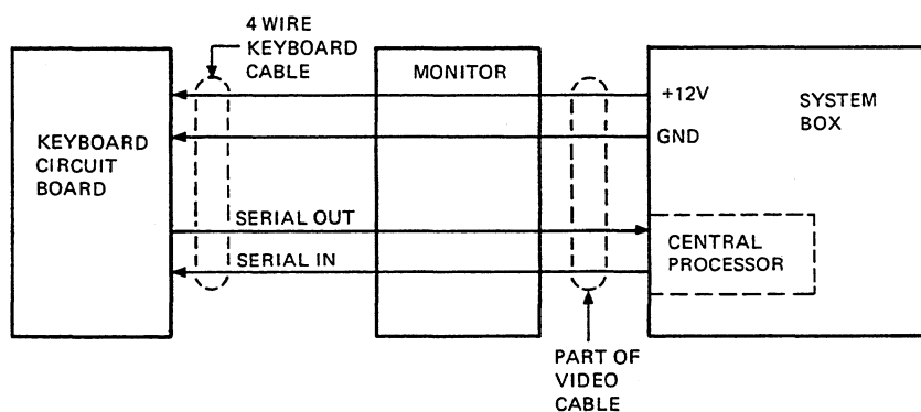
Figure 6-2 Keyboard Cable Connections
