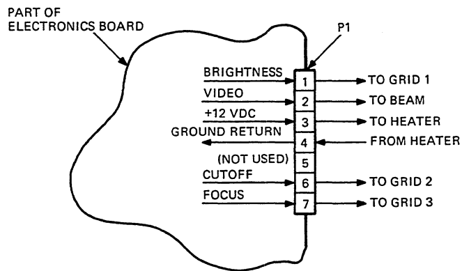
Figure 8-8 Monitor Module P1 Pin-out
