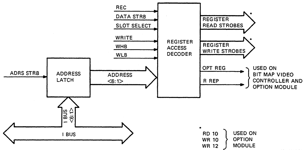
Figure 7-7 CTI BUS Register Access Circuit Operation
