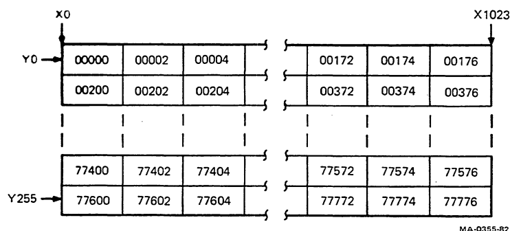
Figure 7-4 Video Memory Bit Map Layout
