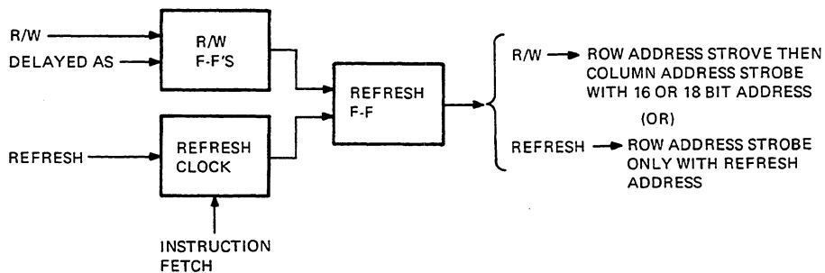
Figure 5-27 Refresh-R/W Arbitration
