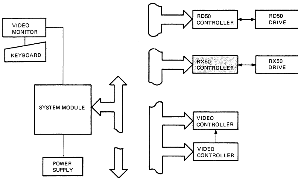
Figure 9-1 RX50 Controller Module System Relation
