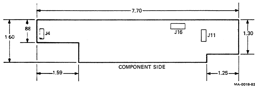
Figure 10-29 Motor Control Module Connector Locations
