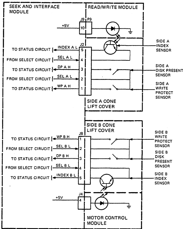
Figure 10-17 Sensor Detail
