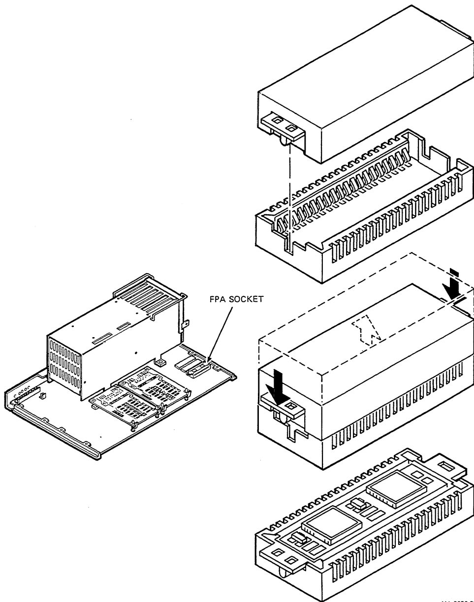
Figure 2-11 Installing the Floating Point Adapter
