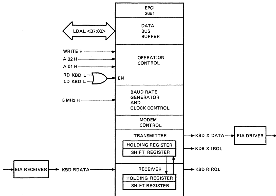
Figure 5-29 Keyboard Interface
