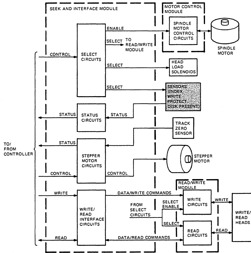
Figure 10-17 Sensor Detail
