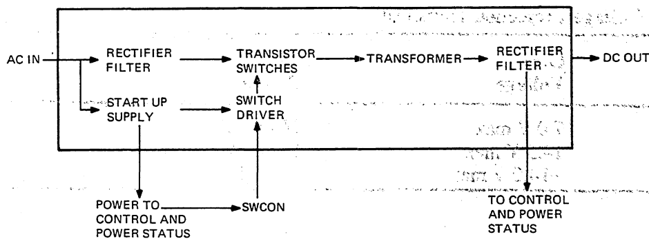
Figure 13-6 Power Conversion
