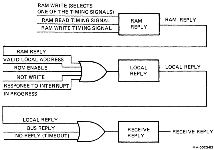
Figure 5-10 Reply
