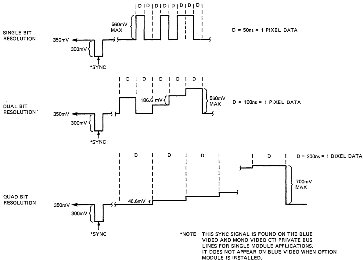
Figure 7-21 Nonmapped Video Signal Characteristics
