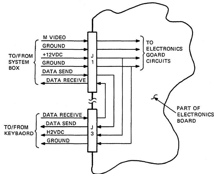
Figure 8-4 Monochrome Monitor System Communications Diagram
