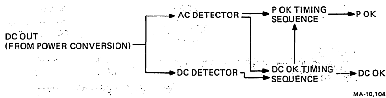
Figure 13-8 Power Status
