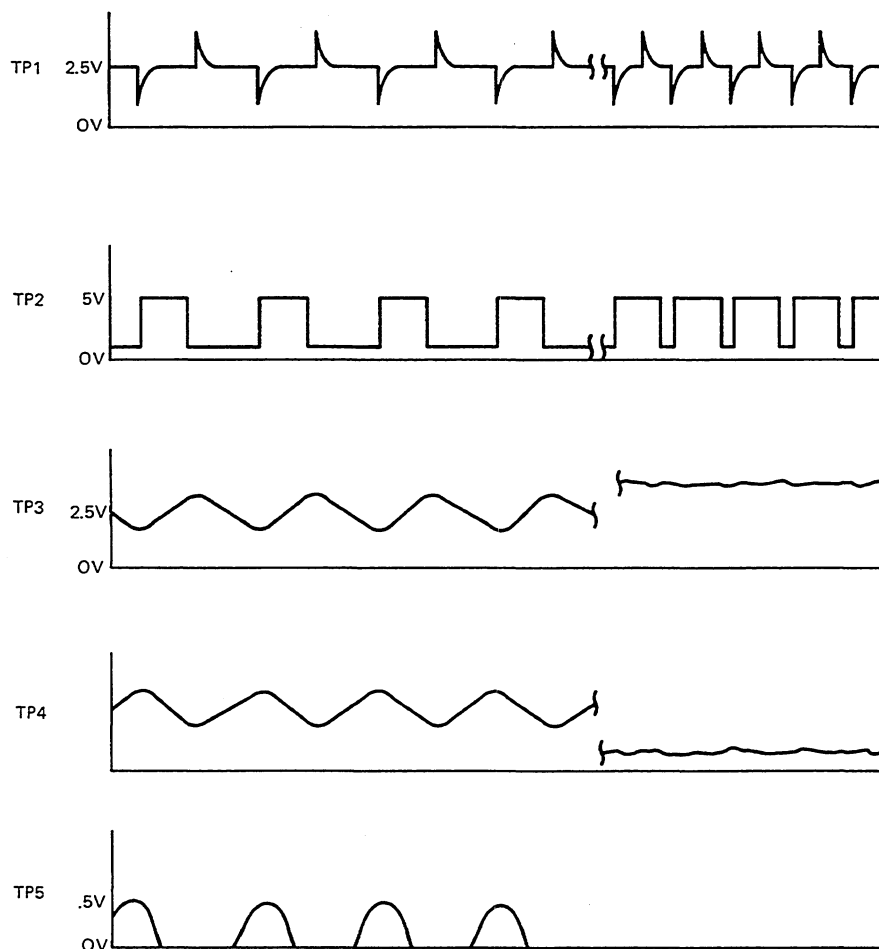
Figure 10-13 Motor Control Wave Forms
