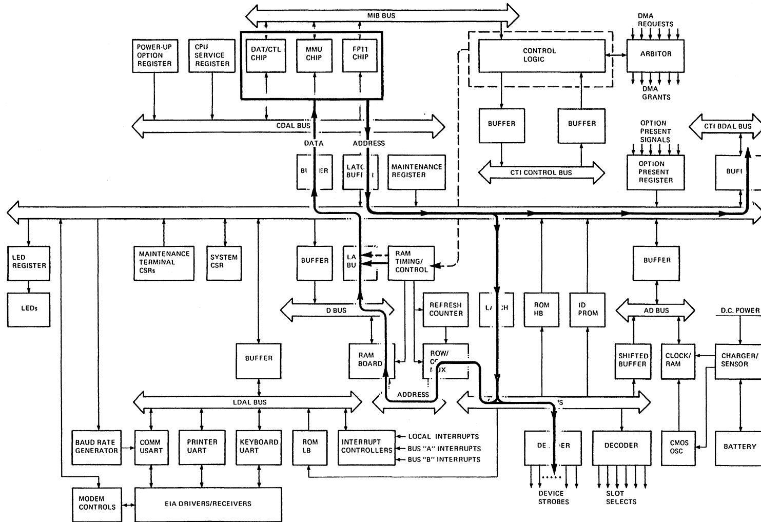
Figure 5-18 CPU Read from RAM
