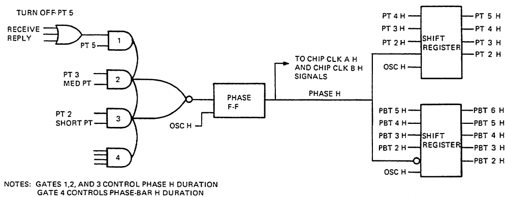
Figure 5-7 Phase Signal Duration Functional Diagram
