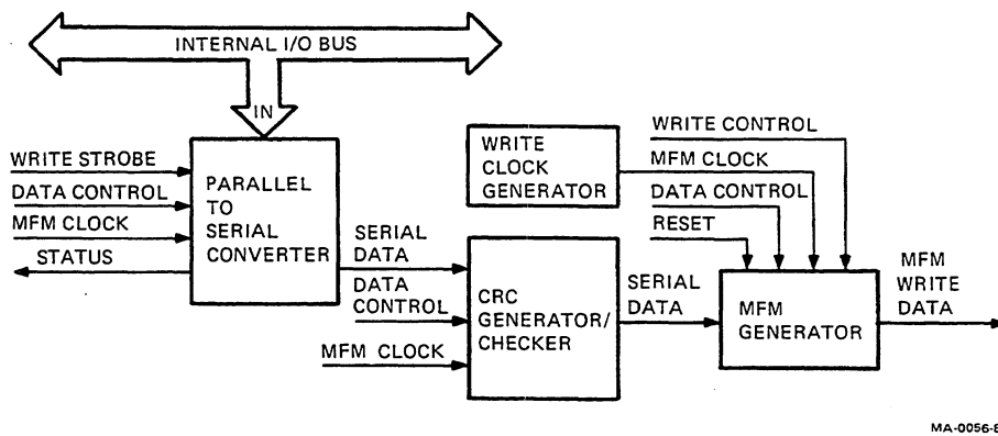
Figure 11-7 MFM Write Data Circuits
