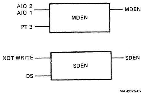
Figure 5-12 Master and Slave Drive Enable
