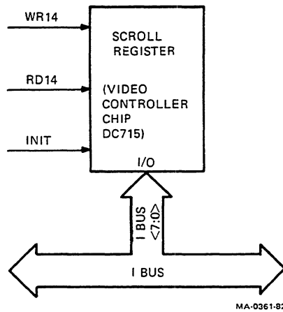
Figure 7-11 Scroll Register Operation
