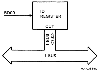
Figure 7-8 ID Register Operation
