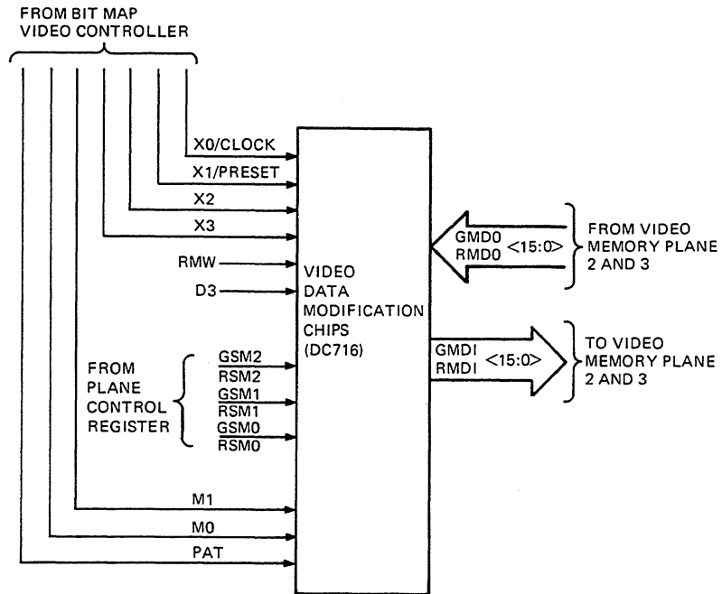
Figure 7-26 Video Data Update Circuit Operation (Option Module)
