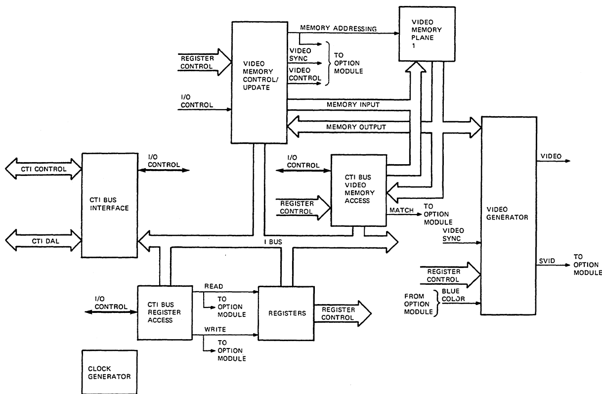
Figure 7-3 Bit Map Video Controller Block Diagram
