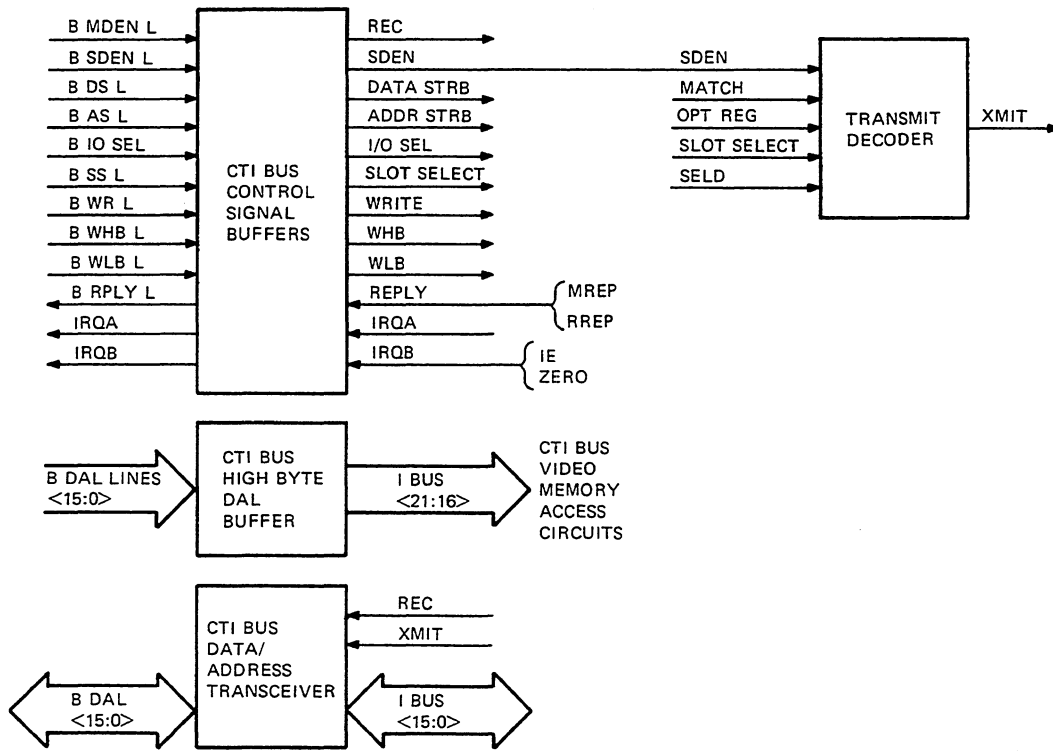
Figure 7-6 CTI BUS Interface Circuit Operation
