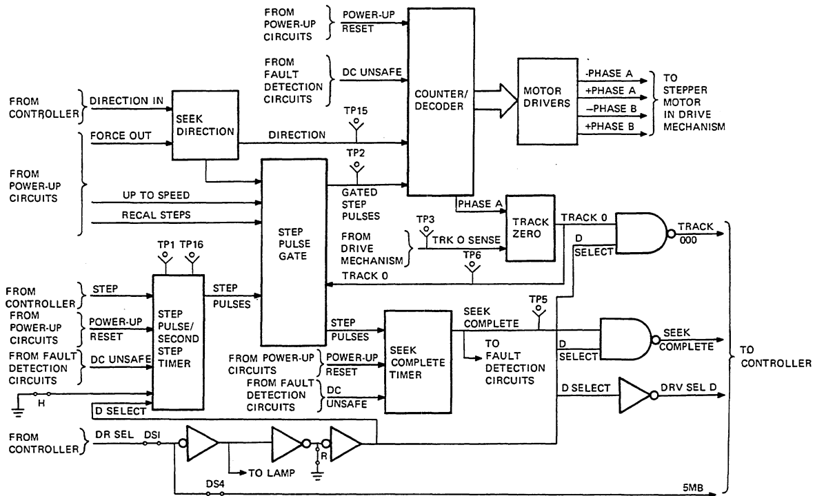
Figure 12-11 Seek Circuit Detail
