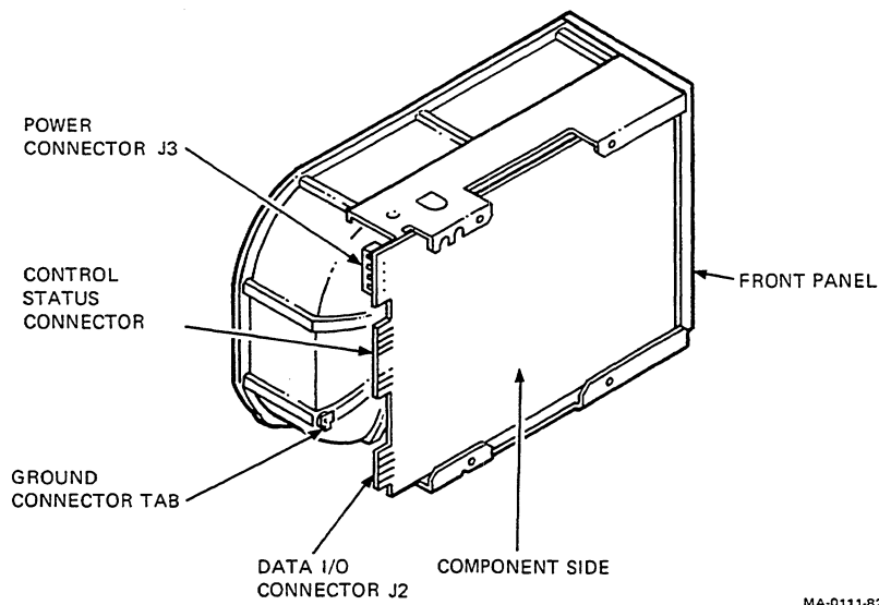
Figure 12-19 I/O Connector Locations
