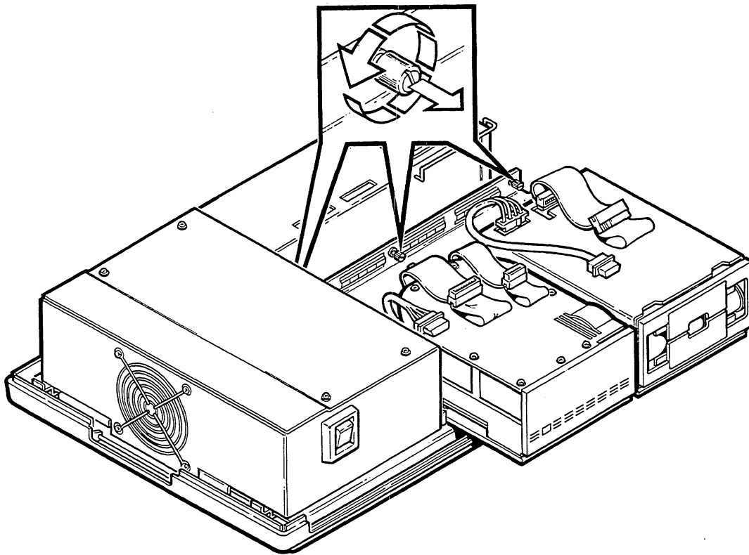
Figure 2-9 Release Thumb Screws
