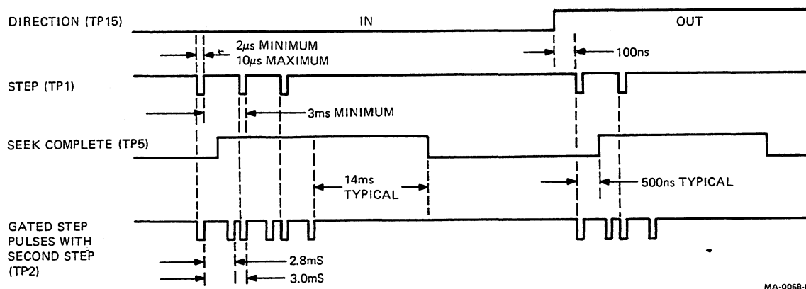
Figure 12-12 Seek Circuit Timing
