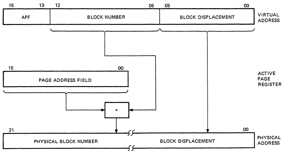
Figure 5-33 Memory Management Relocation
