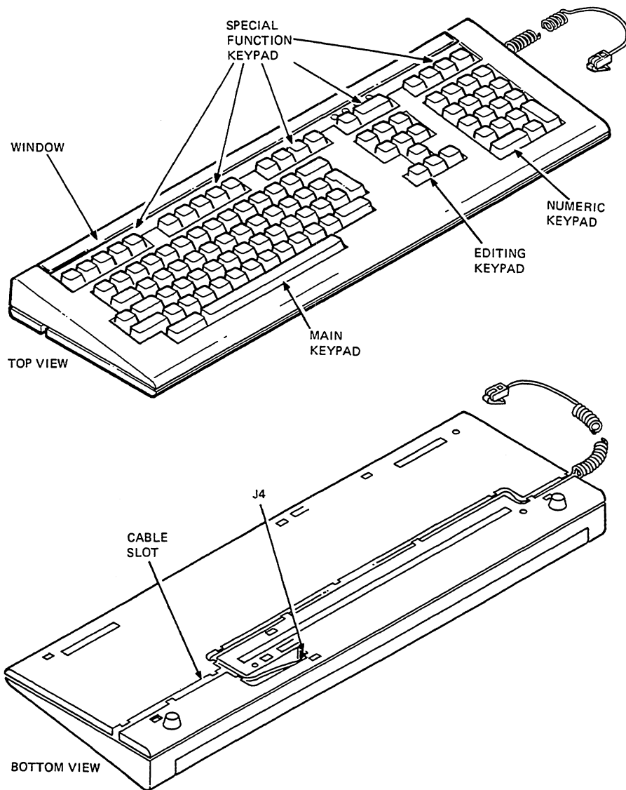
Figure 6-3 LK201 Keyboard
