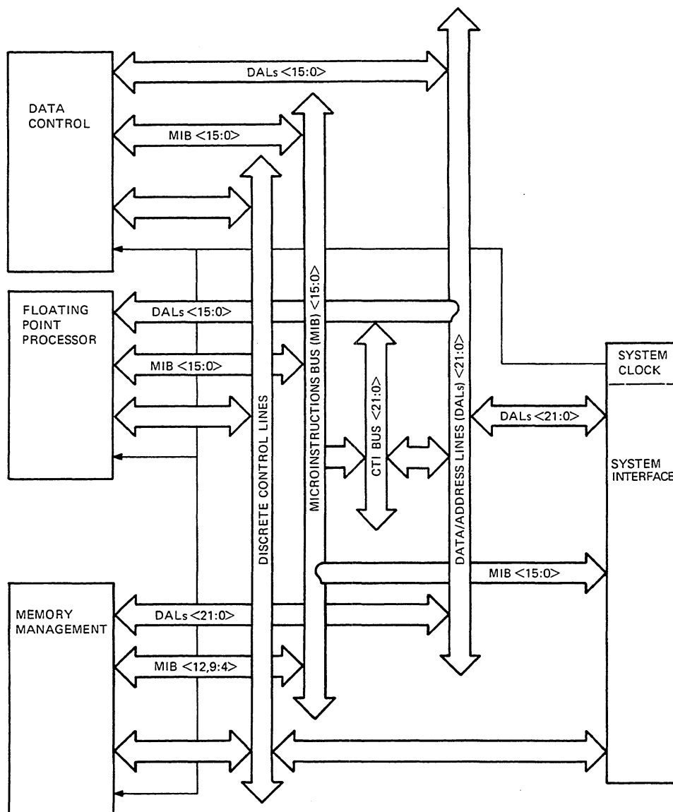
Figure 5-4 CPU Chip Set Communication
