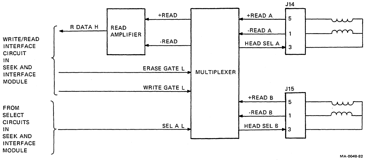
Figure 10-25 Read Circuit Detail
