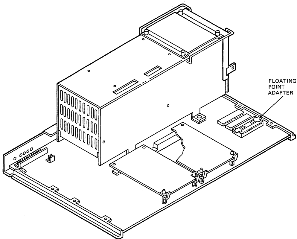
Figure 5-34 Floating Point Adapter Socket Location
