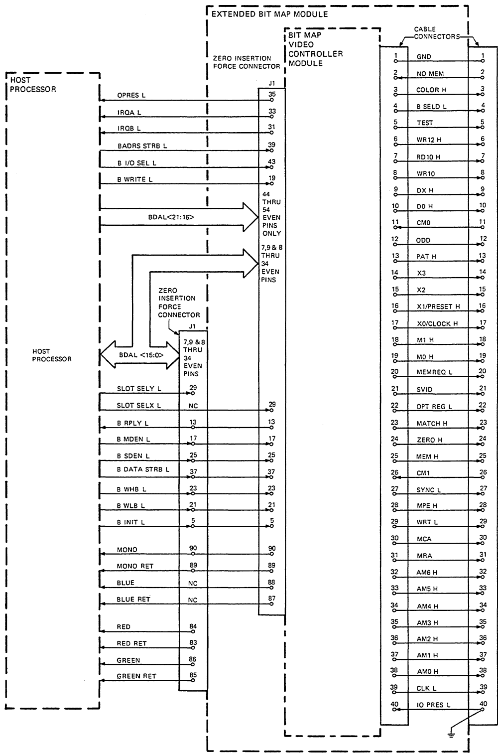
Figure 7-29 Bit Map Video Controller and Extended Bit Map Modules I/O Signal Flow
