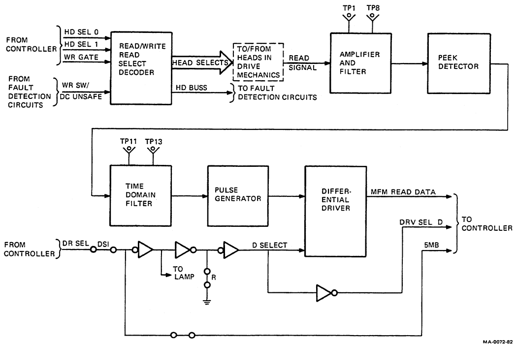
Figure 12-16 Read Circuit Detail
