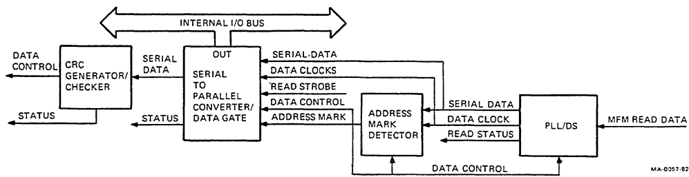
Figure 11-8 MFM Read Data Circuits
