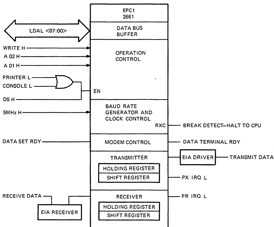
Figure 5-30 Printer Interface
