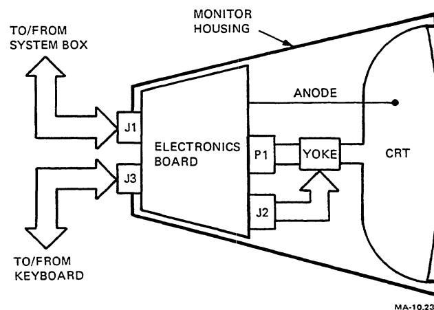
Figure 8-3 Monochrome Monitor Block Diagram
