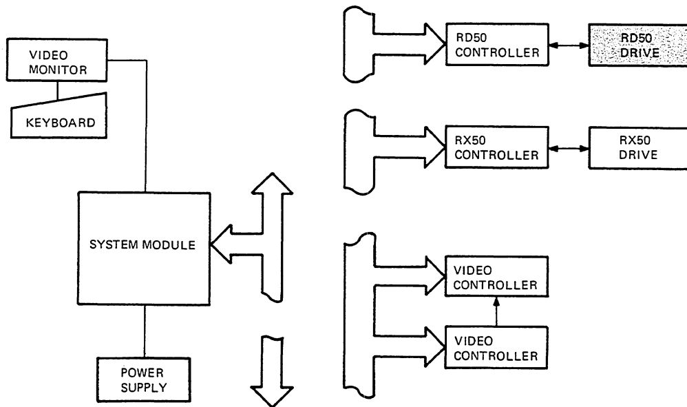
Figure 12-1 RD50 Hard Disk Drive System Relation
