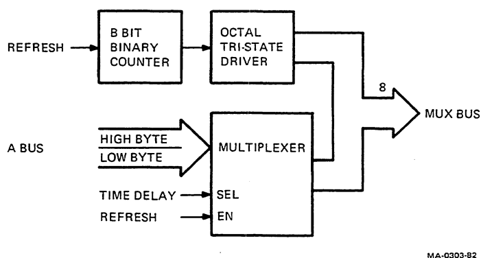
Figure 5-28 RAM Address Multiplexer
