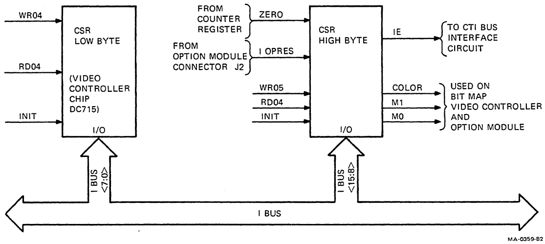
Figure 7-9 CSR Register Operation
