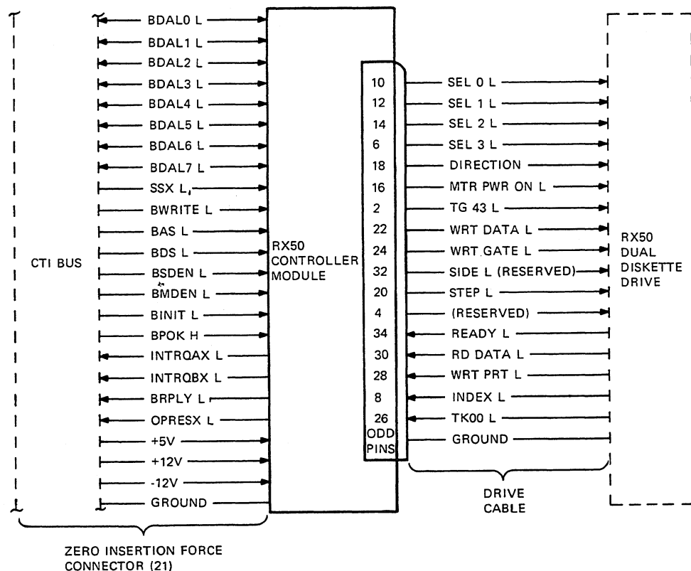
Figure 9-9 RX50 Controller Module Interface Signal Flow
