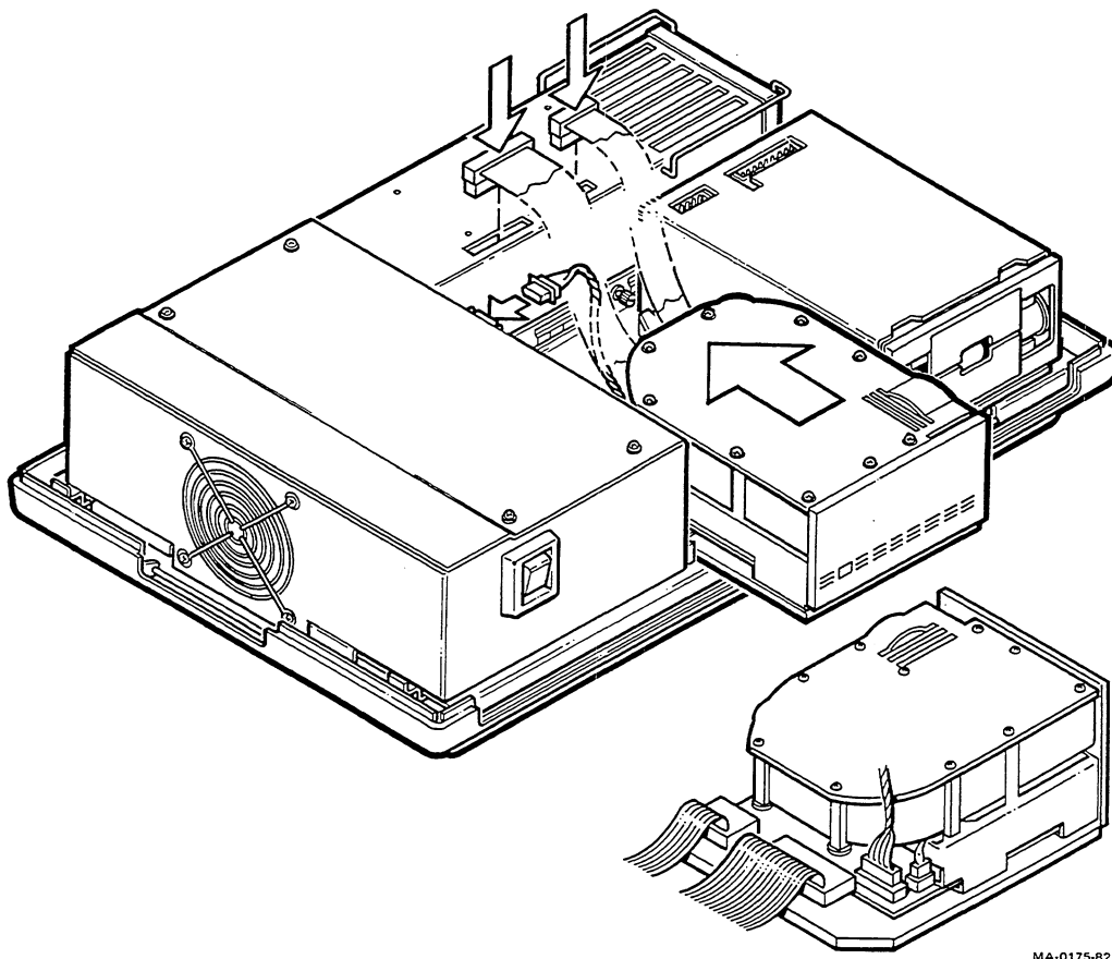
Figure 2-6 RD50 Hard Disk Drive Installation
