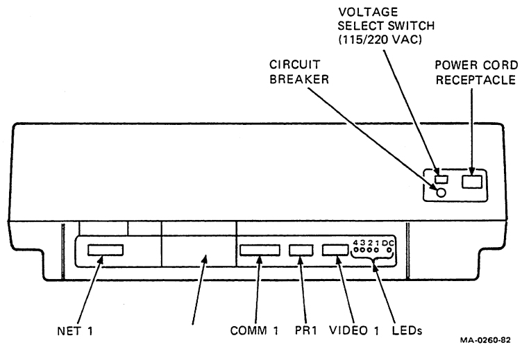
Figure 3-1 System Unit Front Panel
