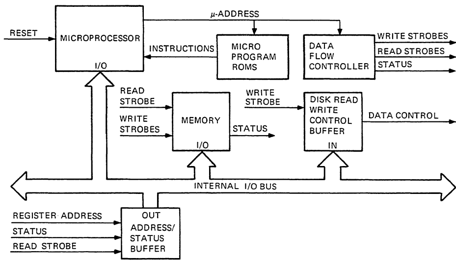
Figure 11-5 Microprocessor Control Circuits
