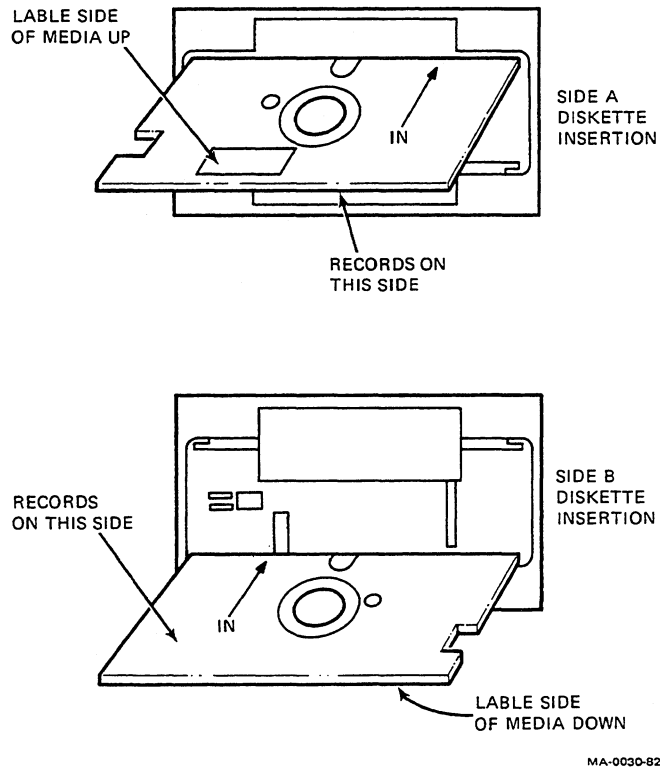
Figure 10-6 Inserting Diskette
