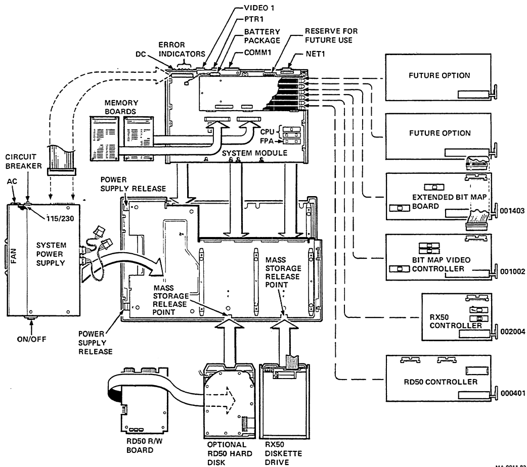
Figure 4-1 Physical Component Block Diagram
