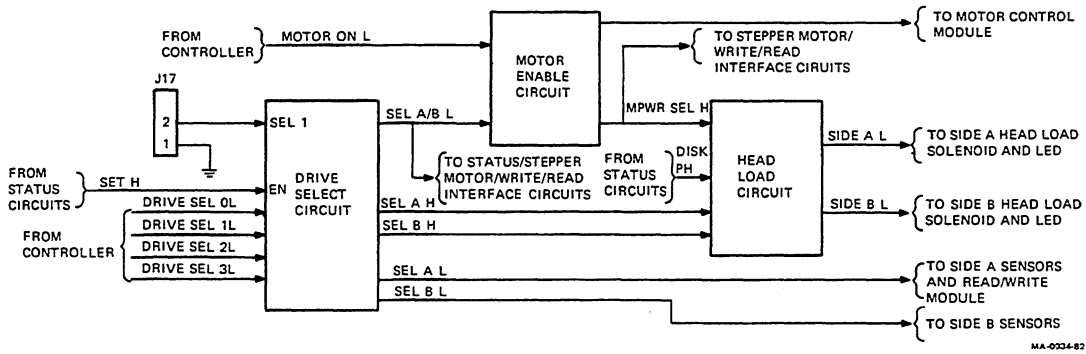
Figure 10-11 Select Circuit Detail
