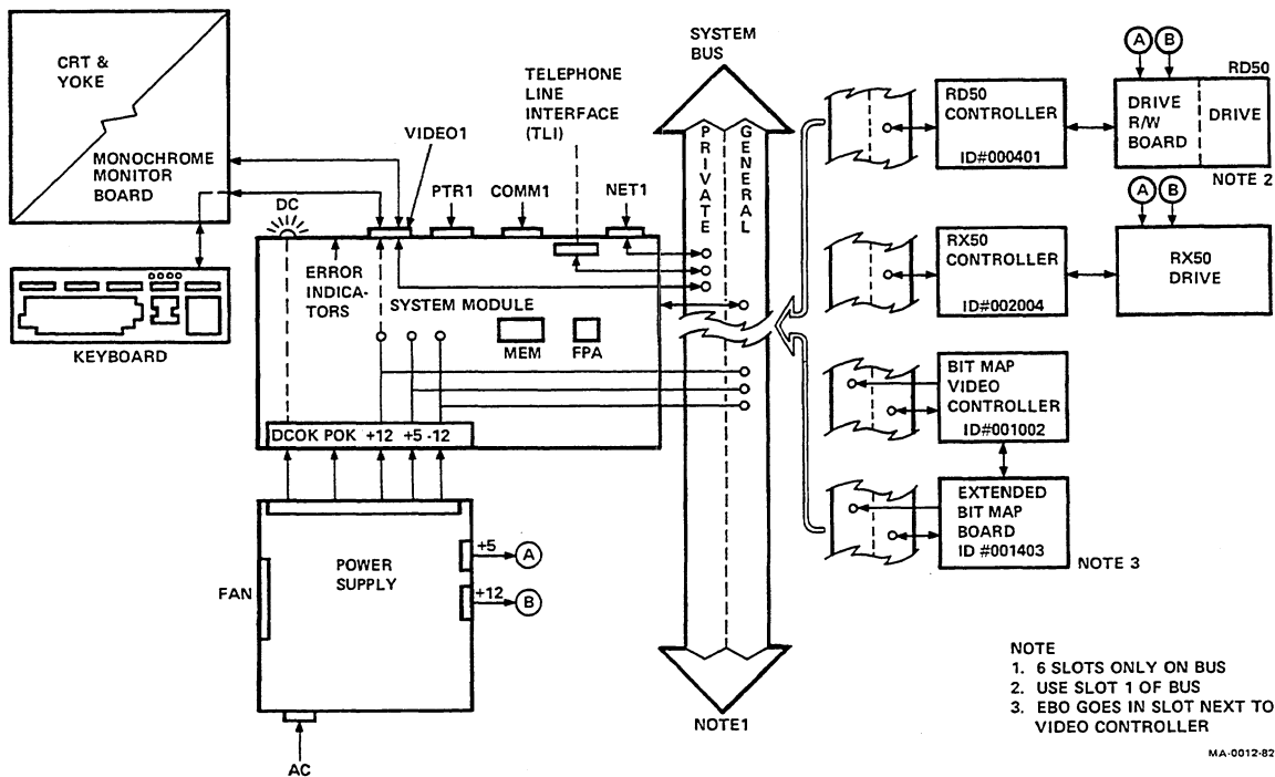
Figure 4-2 Functional System Block Diagram
