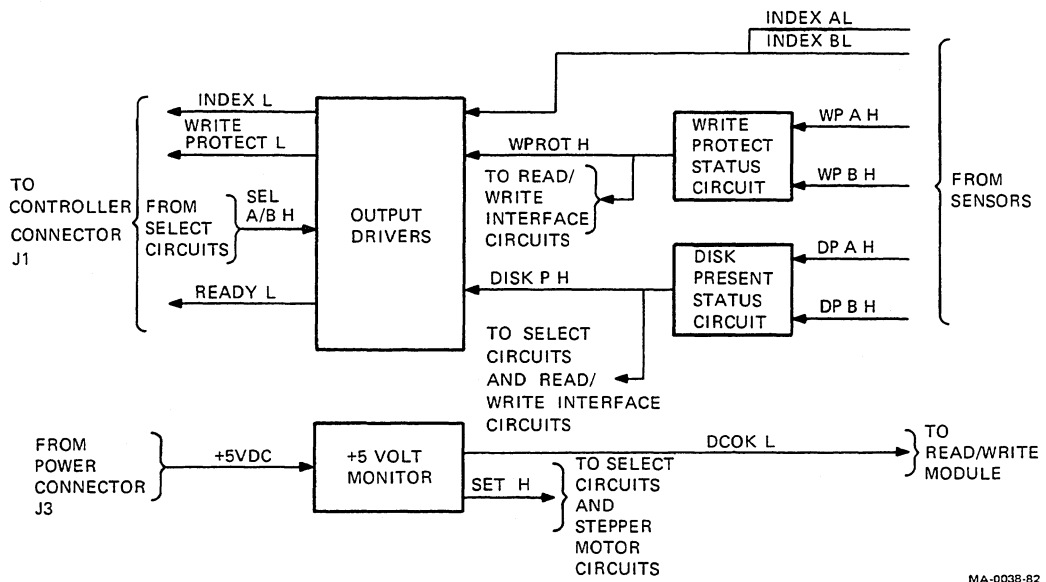
Figure 10-15 Status Circuit Detail
