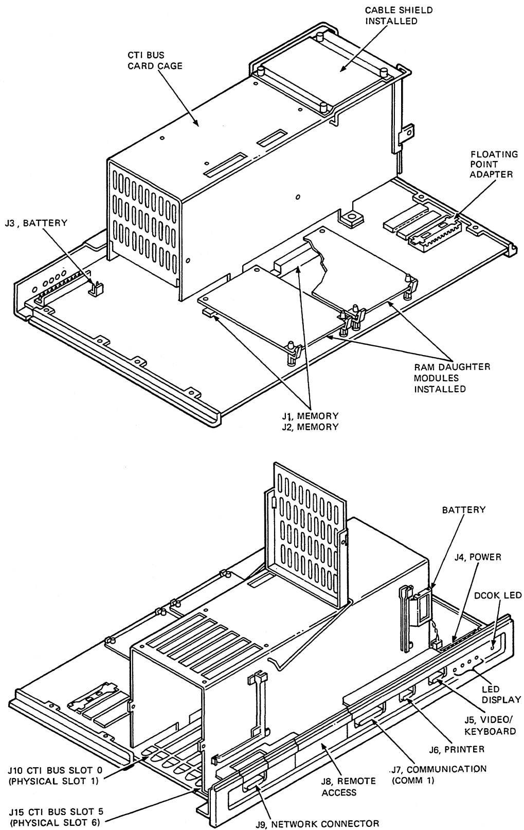
Figure 5-2 System Module
