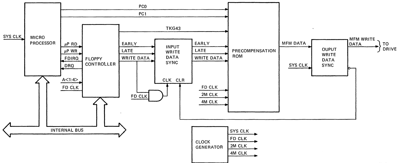
Figure 9-7 MFM Write Data Interface Circuits
