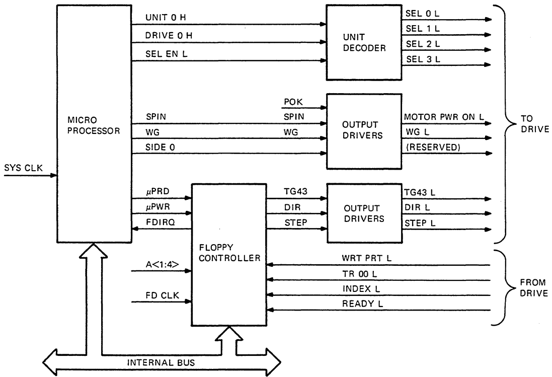
Figure 9-6 Disk Control and Status Interface Circuits
