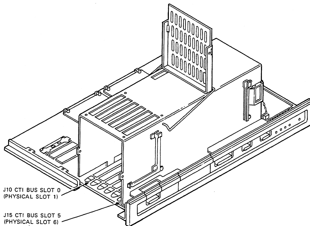
Figure 5-35 CTI BUS Option Slots
