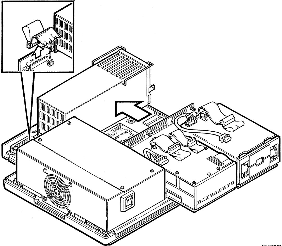
Figure 2-10 Removing the System Module
