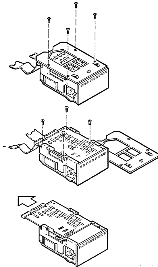
Figure 12-22 Assembly and Disassembly
