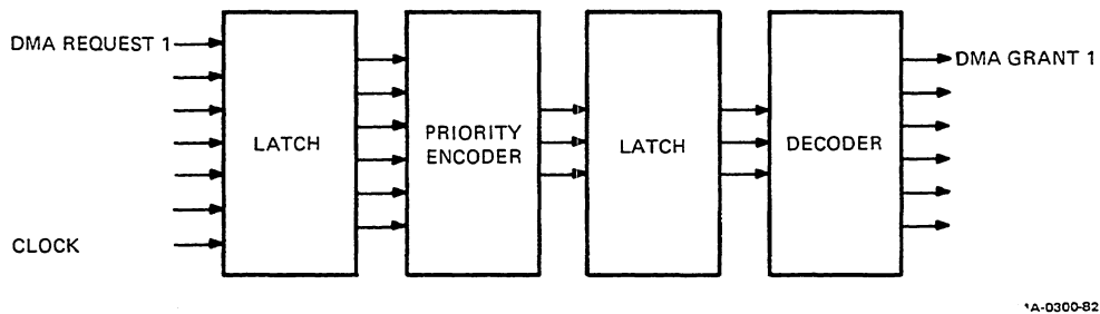
Figure 5-25 DMA Arbitor
