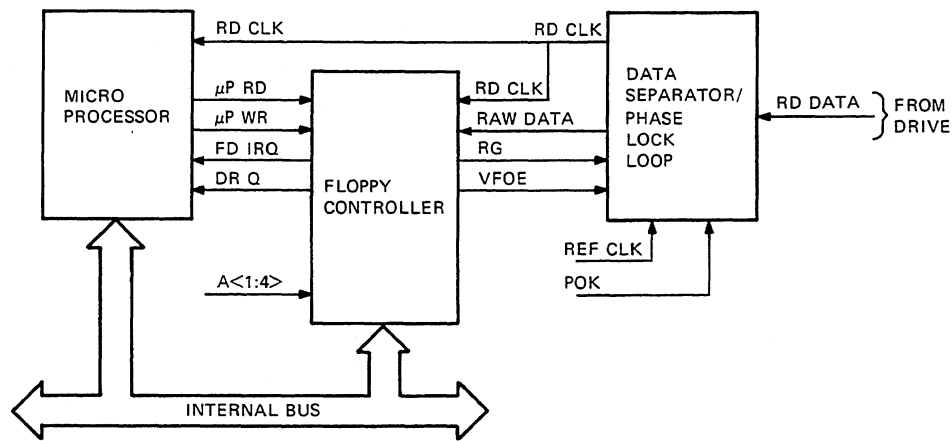
Figure 9-8 MFM Read Data Interface Circuits
