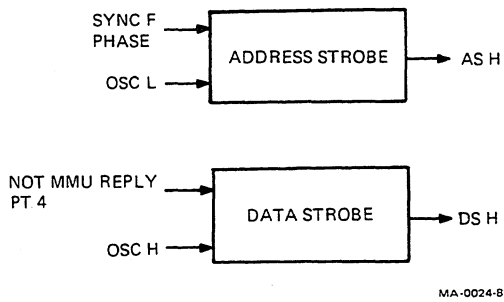
Figure 5-11 Address and Data Strobe
