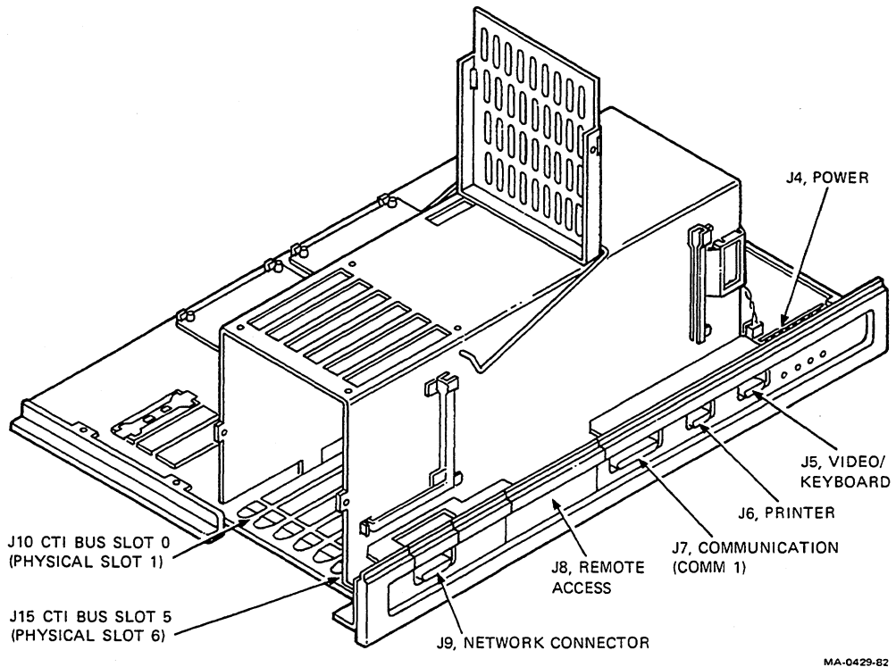
Figure 5-37 Connector Placement
