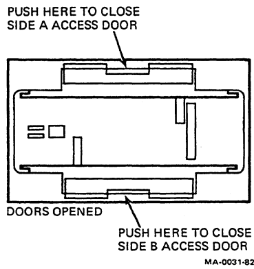
Figure 10-7 Closing Access Doors
