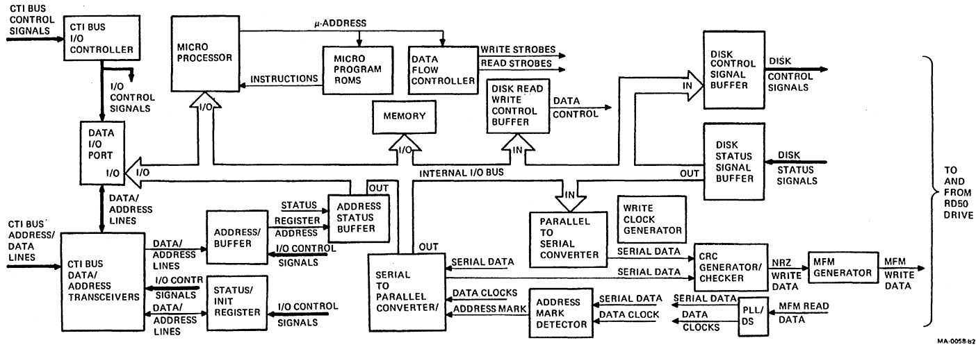
Figure 11-9 RD50 Controller Data Flow Diagram
