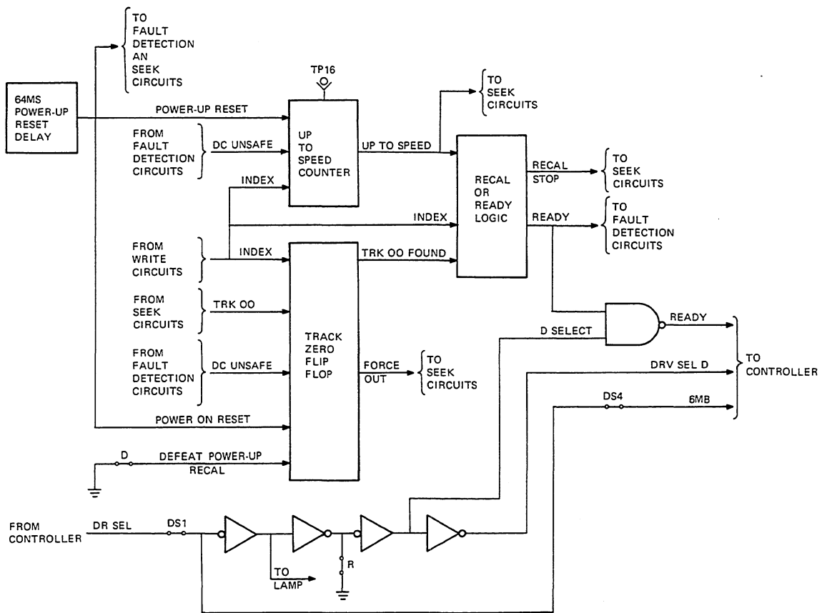
Figure 12-8 Power-up Circuit Detail
