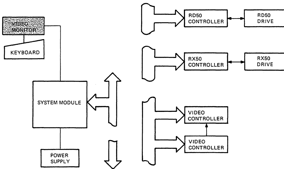
Figure 8-1 System Block Diagram
