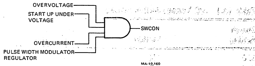
Figure 13-5 Protection
