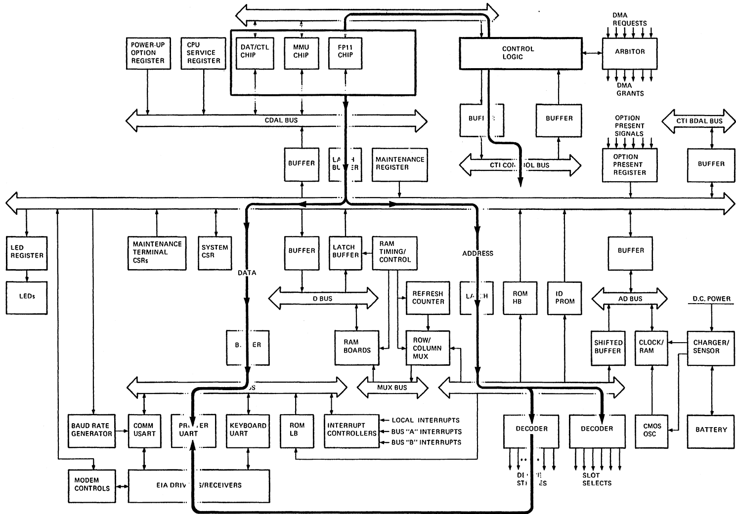
Figure 5-16 CPU Writing to I/O Device
