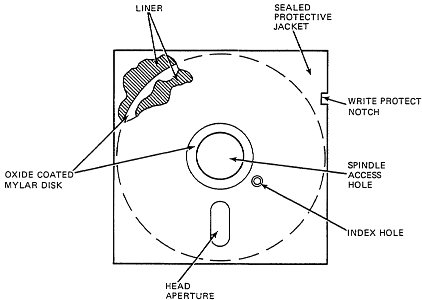
Figure 10-3 The 5.25 Inch Diskette
