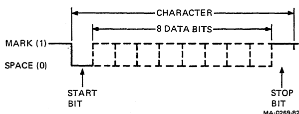
Figure 6-10 Keyboard Transmit and Receive Character Format
