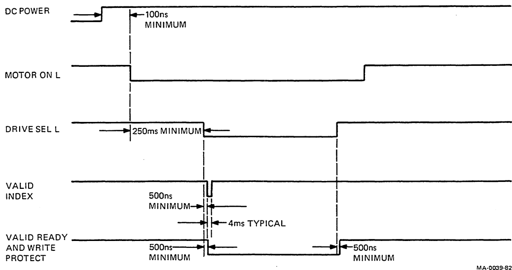
Figure 10-16 Status Circuit Timing Relationships
