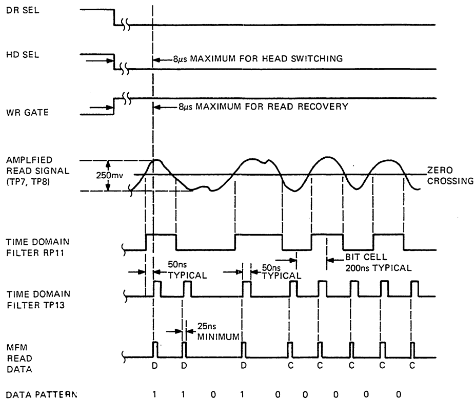
Figure 12-17 Read Data Timing
