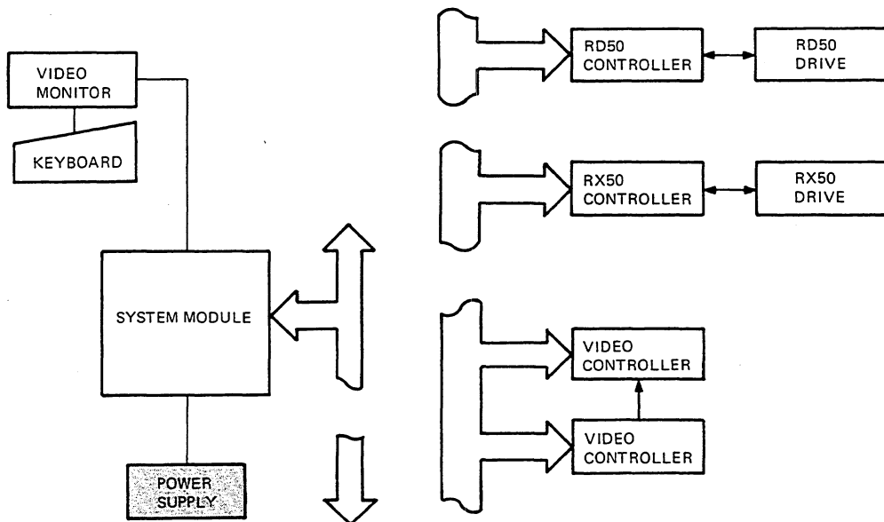
Figure 13-1 System Functional Block Diagram
