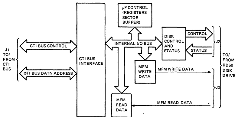
Figure 11-3 RD50 Controller Block Diagram
