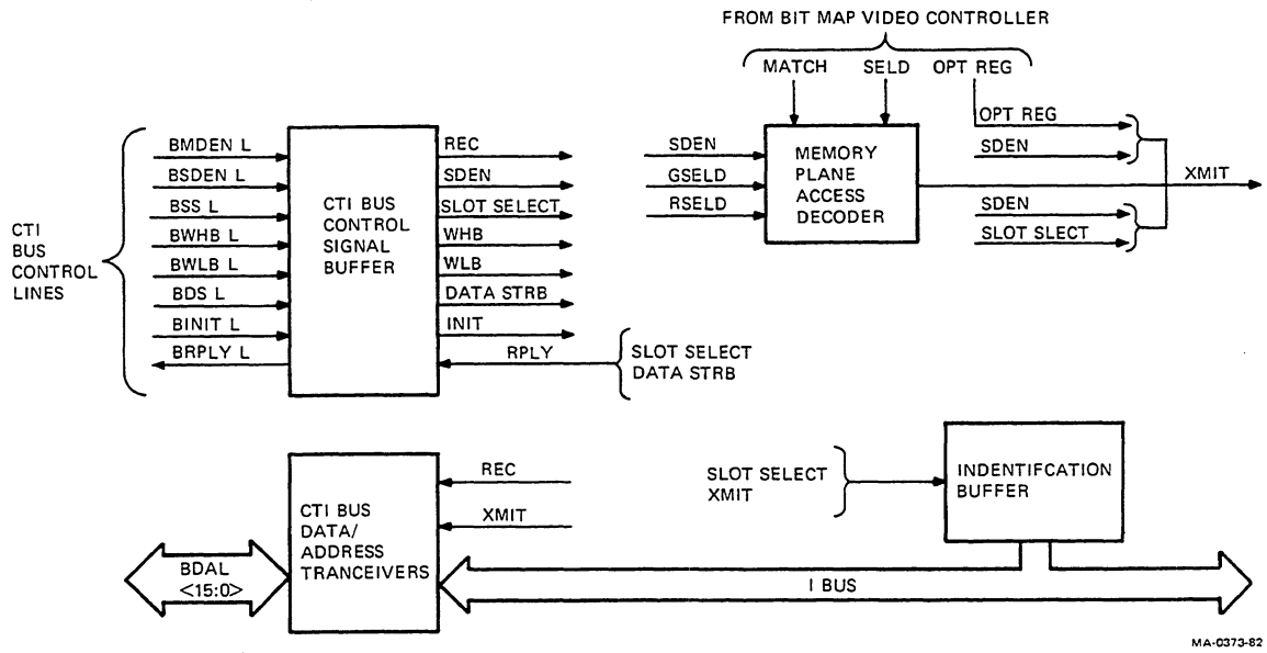
Figure 7-23 CTI BUS Interfaced Circuit Operation (Option Module)
