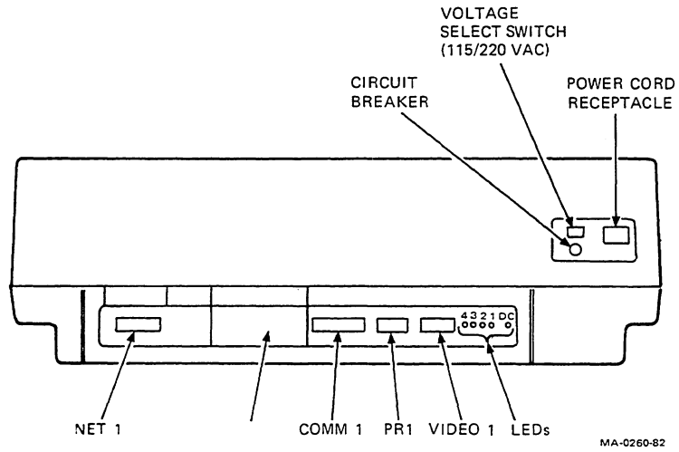
Figure 2-1 System Unit Rear Panel
