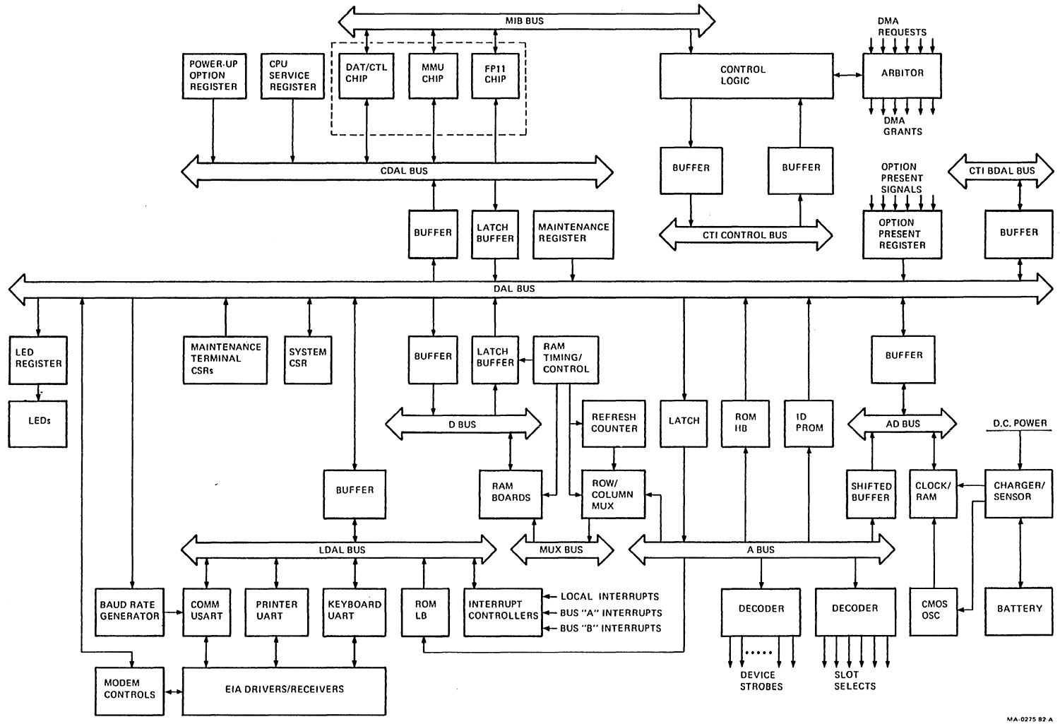
Figure 5-8 System Module Block Diagram
