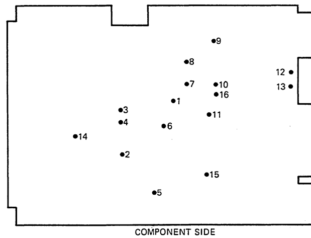
Figure 12-21 R/W Module Test Point Locations
