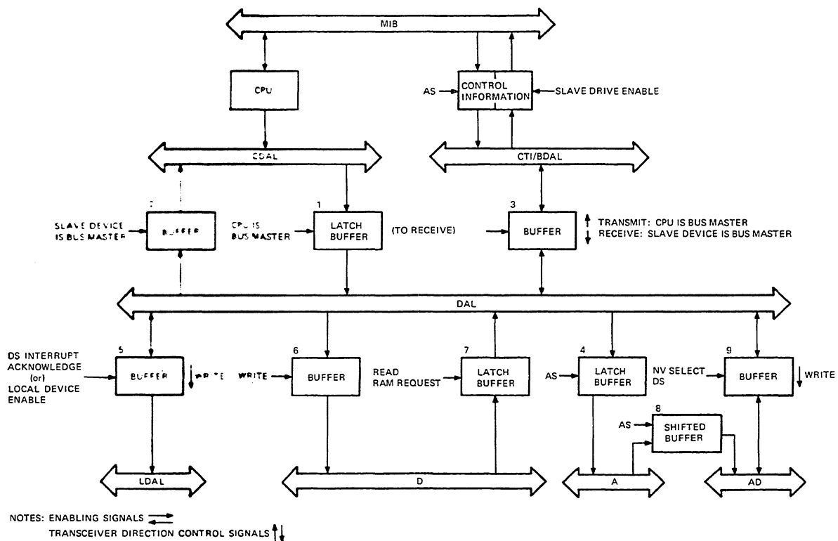
Figure 5-13 System Block Diagram with Bus Interfaces
