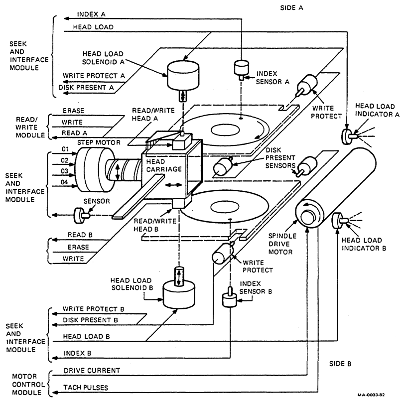
Figure 10-10 Mechanical Operation Detail
