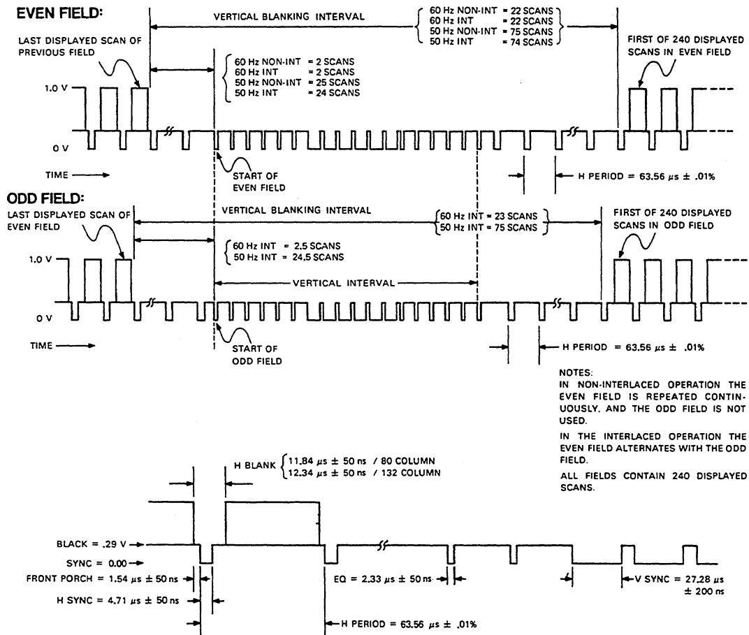
Figure 8-6 Composite Video Sync Timing Diagram
