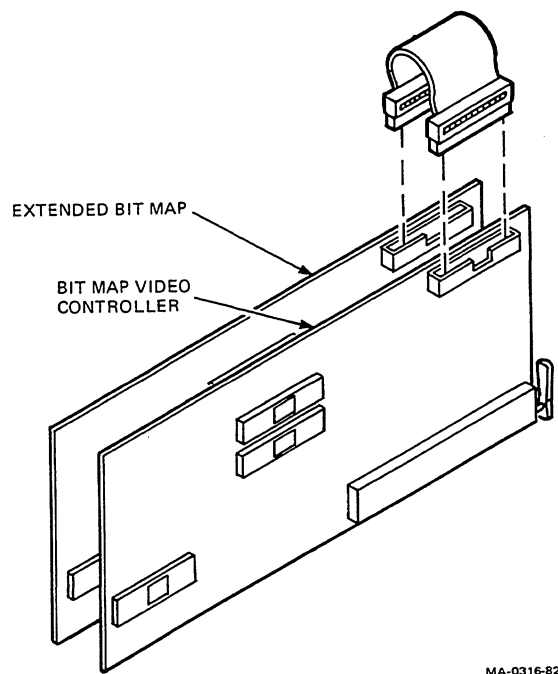
Figure 7-2 Bit Map Video Controller and Extended Bit Map Modules
