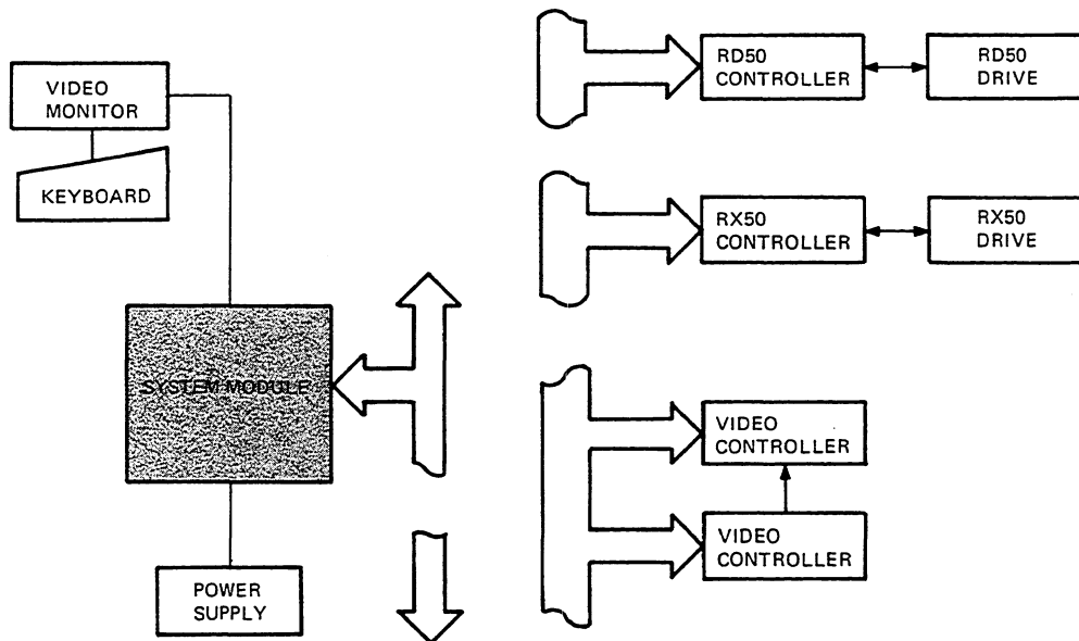
Figure 5-1 System Block Diagram
