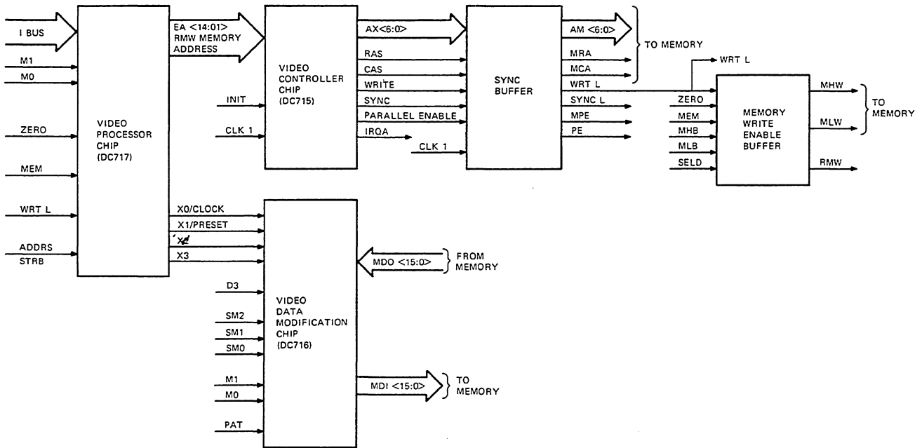
Figure 7-18 Video Memory Control and Update Circuit Operation
