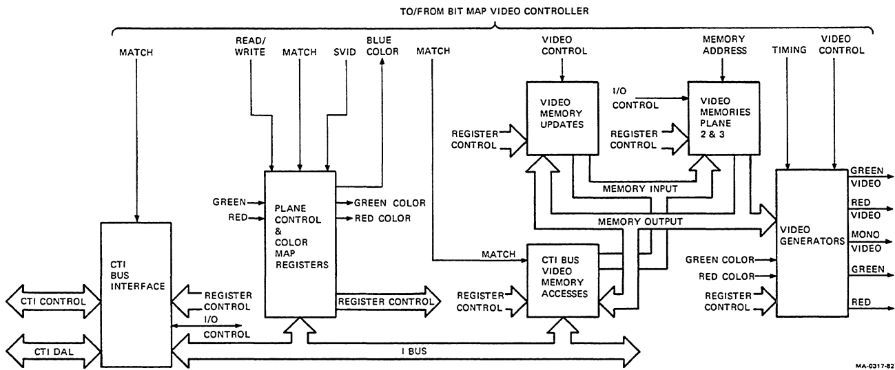
Figure 7-5 Extended Bit Map Block Diagram
