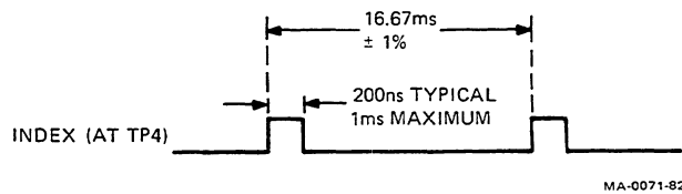
Figure 12-15 Index Signal Timing
