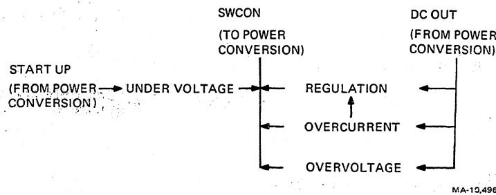
Figure 13-7 Protection Block Diagram
