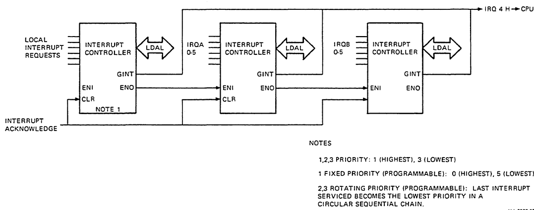
Figure 5-23 Functional Interrupt Control Circuit
