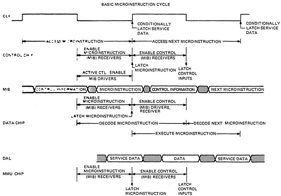
Figure 5-5 Basic Microinstruction Cycle
