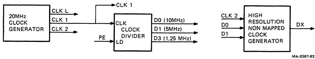
Figure 7-17 Clock Generator Circuit Operation
