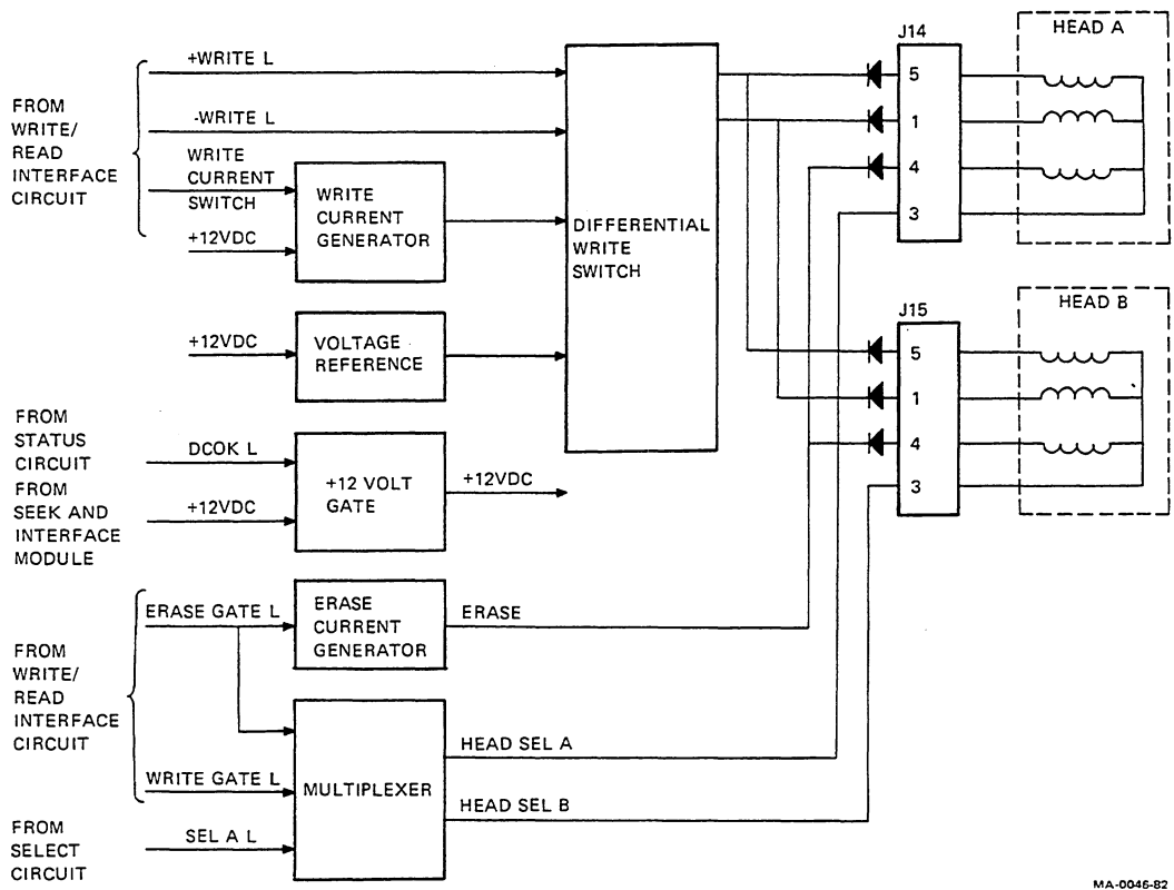
Figure 10-23 Write Circuit Detail
